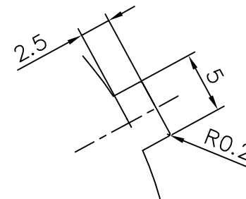
KEYWAY DETAIL
