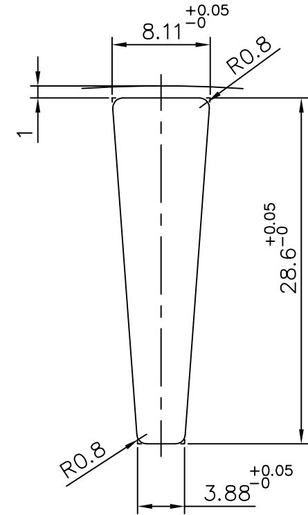
DETAIL - 'X'
