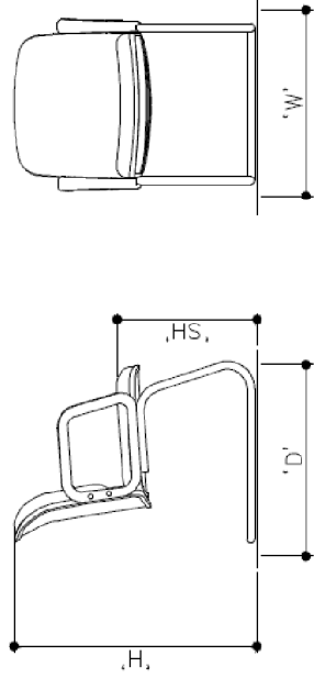
Chair for visitors: W-55cm, D-61cm, H-80.5 cm, SH-44 cm, Tolerance- \pm 0.5 cm
