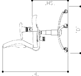
Chair for Executives & Conf. hall W-70cm, D-70cm, H-90 to 102.5cm, SH-44 to 56.5cm Tolerance- \pm 0.5 cm
