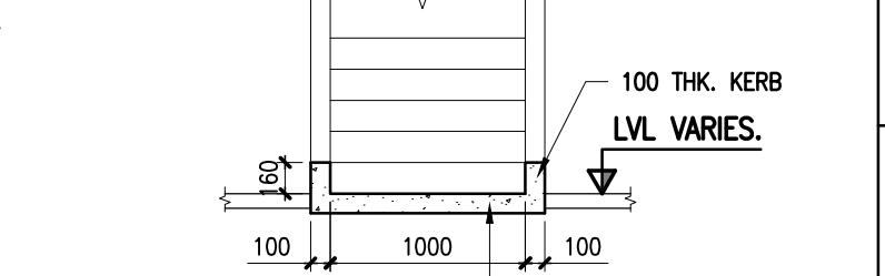
DETAIL-D4 (TYP. DETAIL OF TOE DRAIN)
