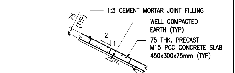
DETAIL-D3 (TYP. DETAIL OF TOE DRAIN)
