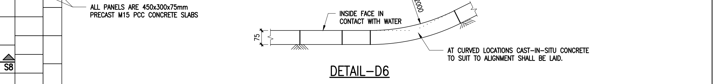
DETAIL-D6 (TYP. DETAIL OF TOE DRAIN)
