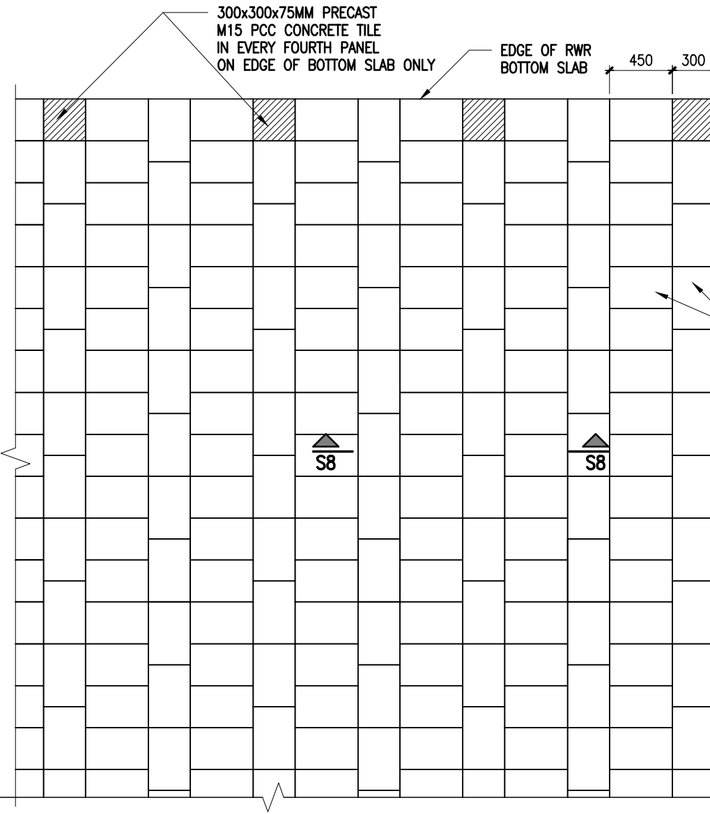
TYPICAL PLAN OF PRECAST CONCRETE SLAB LAYING
