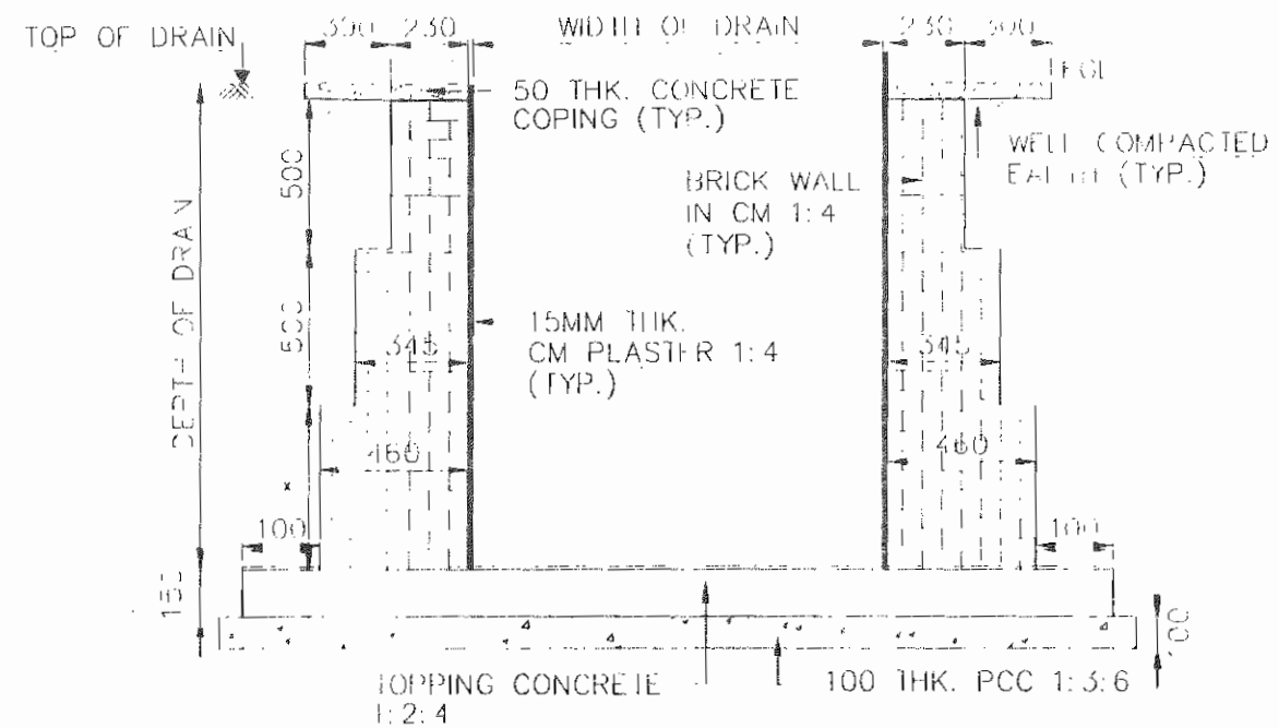
TYP. DETAILS OF RECT. OPEN DRAIN MARKED D1 TO D4 (SCALE 1:25)
