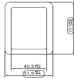
SECTION G-G
