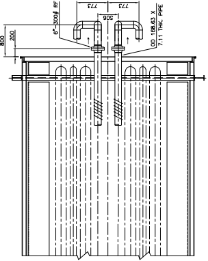
SECTION - A2A2 (CRUDE OUTLET TO ECONOMISER COIL)
