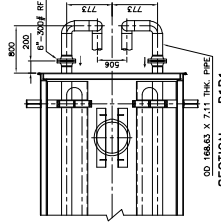
SECTION - B1B1 (CRUDE INLET TO MAIN COIL FROM ECONOMISER COIL)
