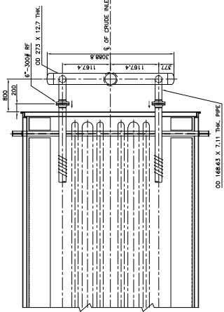
SECTION - A1A1 (CRUDE INLET TO ECONOMISER COIL)
