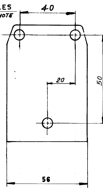
VIEW - P (ALTERNATE MOUNTING DETAILS)
