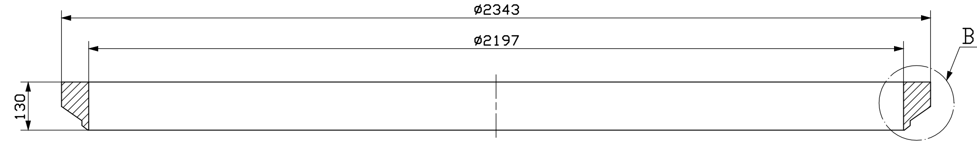
SECTION-AA (1: 10)
