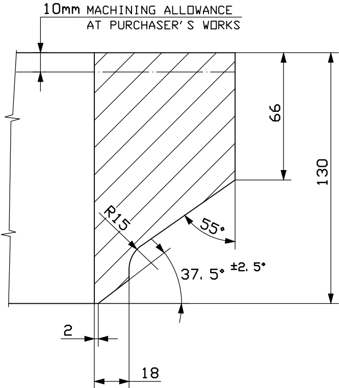
DETAIL-B (1: 2)
