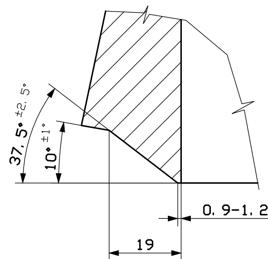
DETAIL-A (1:1)
