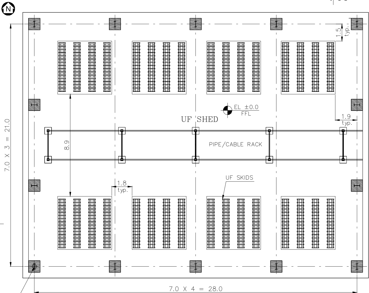
UF SHED LAYOUT - PLAN
