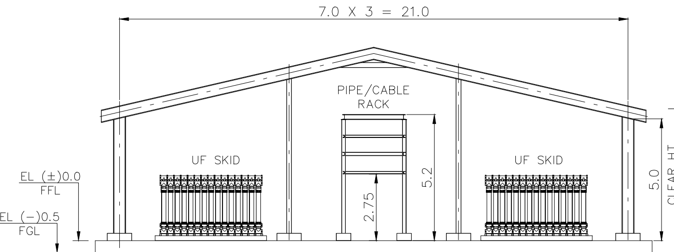
SECTION X-X
