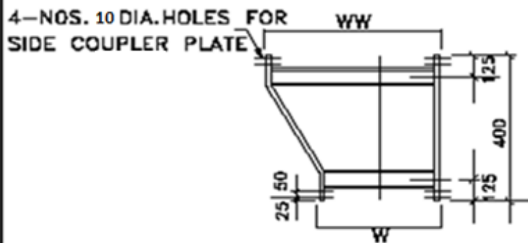
RIGHT HAND REDUCER-PLAN
