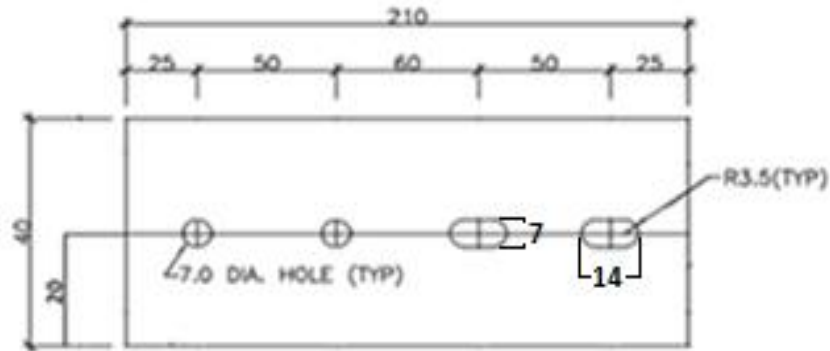
FRP SIDE COUPLER PLATE FOR FRP PERFORATED TYPE TRAYS (50/100W TRAYS)
