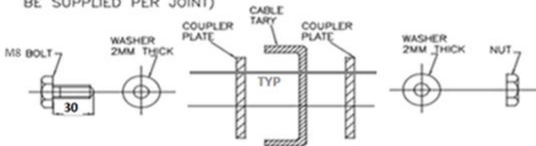
SEQUENCE OF M8 BOLT, WASHER, NUT, COUPLER PLATE & CABLE TRAY FOR TYPICAL CABLE TRAY JOINT
