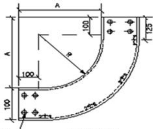
ELEVATION 90° VERTICAL BEND (INSIDE)
