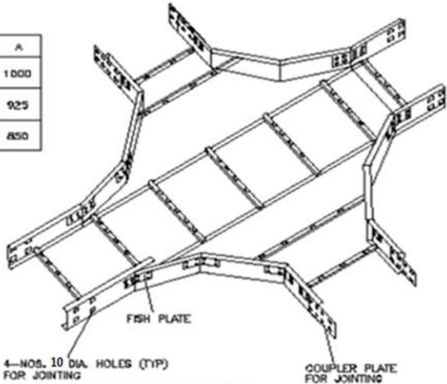
HORIZONTAL CROSS-PLAN
