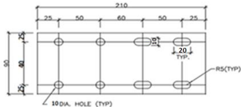
FRP SIDE COUPLER PLATE FOR FRP LADDER/PERFORATED TYPE TRAYS (600/450/300/150W TRAYS)
