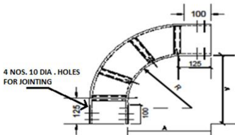
PLAN 90° HORIZONTAL RIGHT BEND
