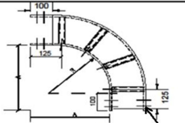
PLAN 90° HORIZONTAL LEFT BEND
