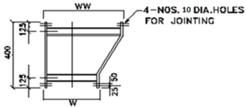
LEFT HAND REDUCER-PLAN
