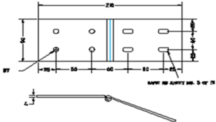
FRP ADJUSTABLE HORIZONTAL SPLICE PLATE
