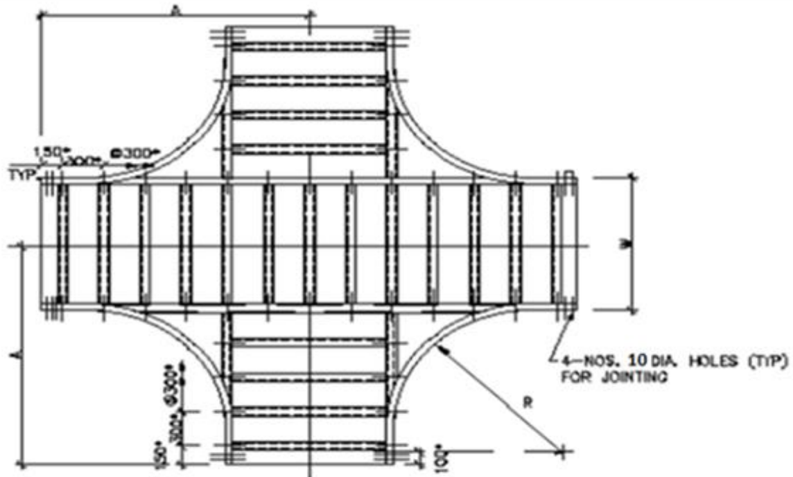
HORIZONTAL CROSS-PLAN
