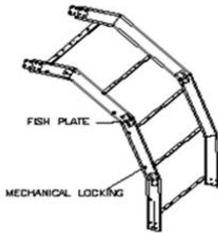
90° VERTICAL BEND (OUTSIDE)
