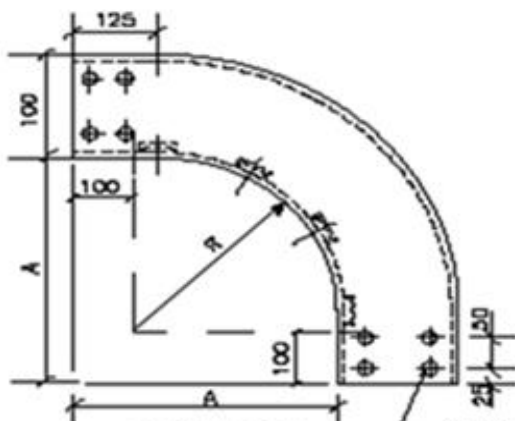
ELEVATION 90° VERTICAL BEND (OUTSIDE)
