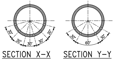
TYP. LATERAL PIPE DETAILS
