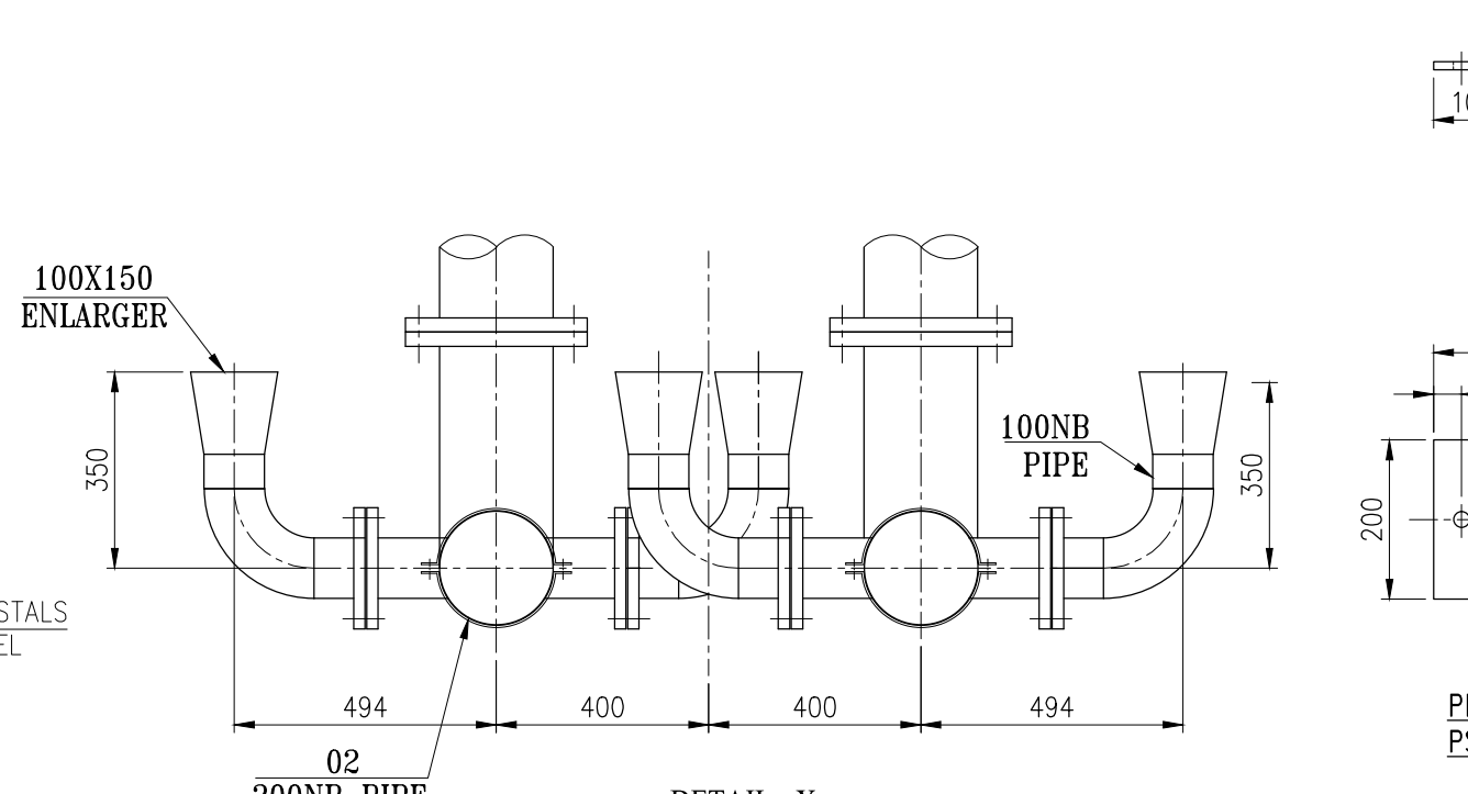
EXTERNAL PIPE SUPPORT LEG FIXING DETAILS
