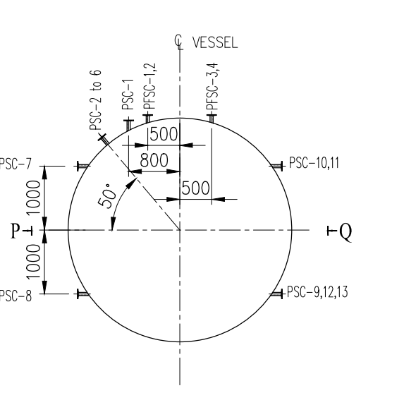
EXTERNAL PIPE SUPPORT LEG FIXING DETAILS
