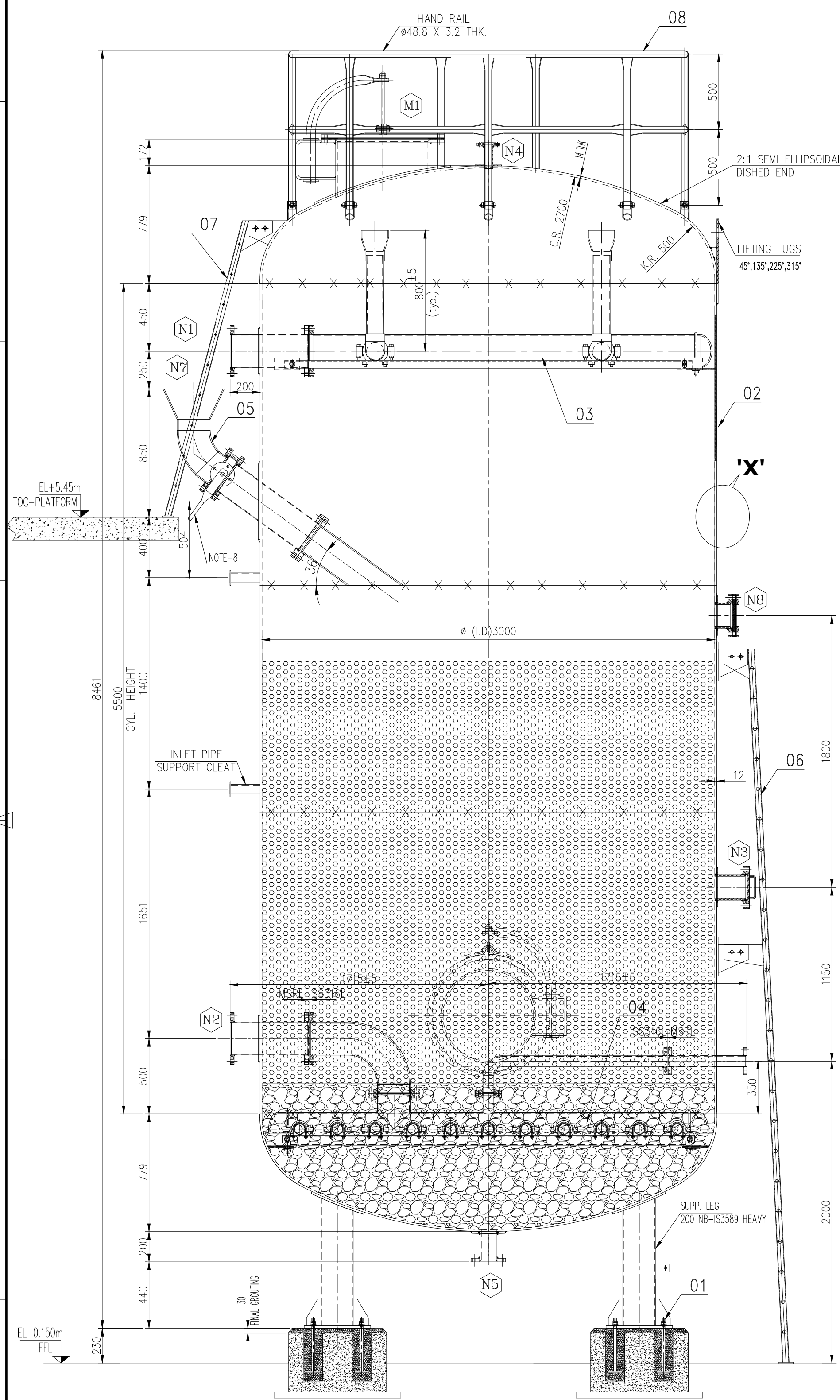
NOZZLE AND LADDER DETAILS :
