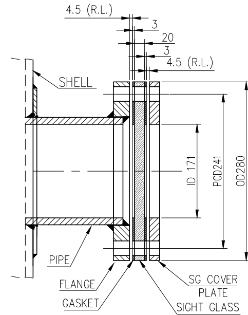
DETAIL - 'Y'
