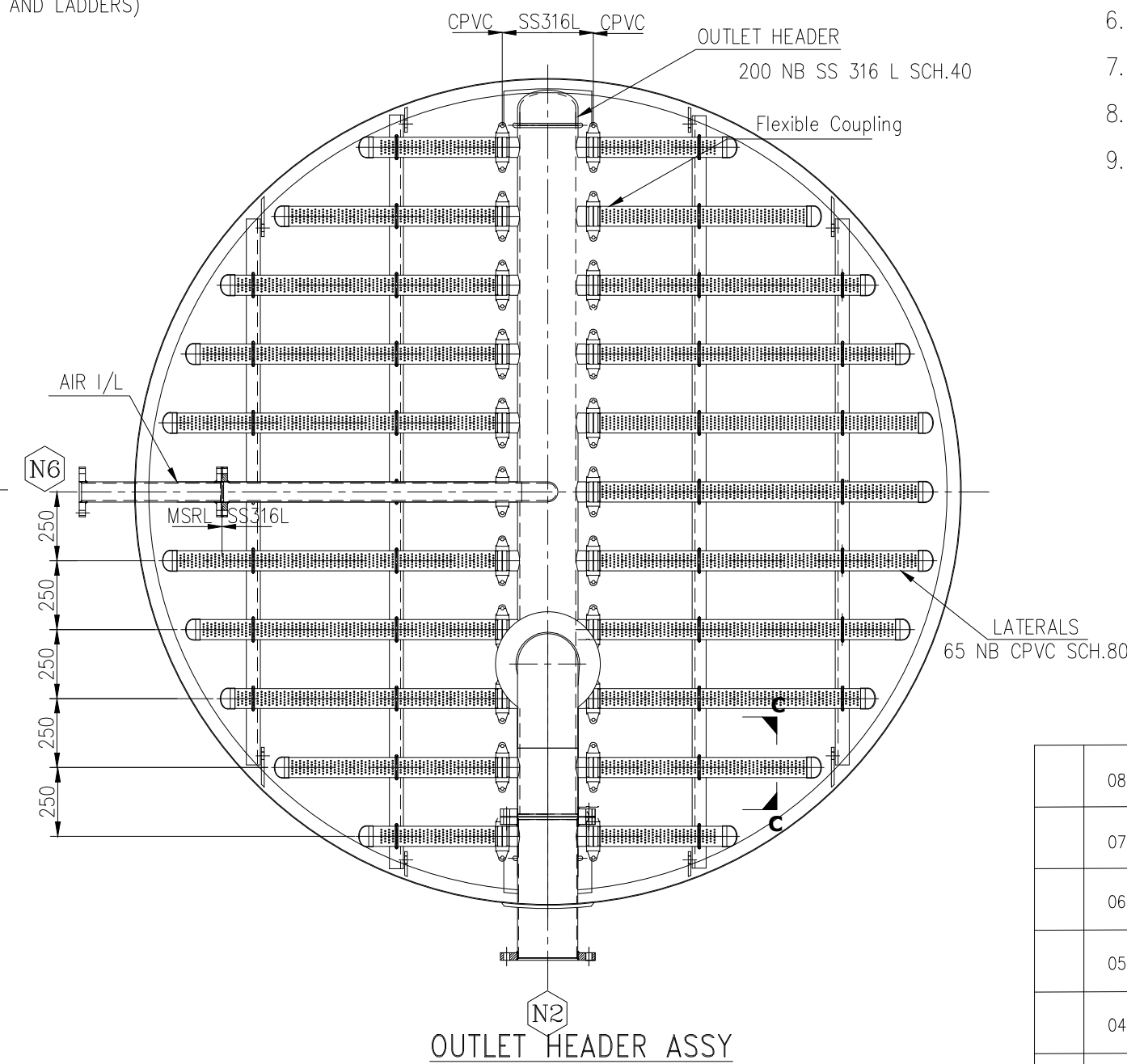
OUTLET HEADER ASSY
