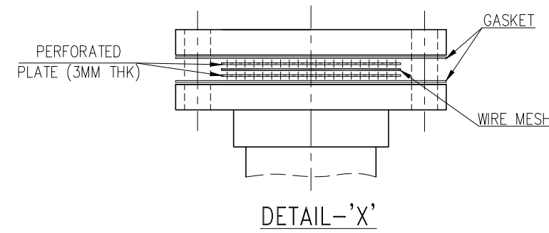
DETAIL - 'X'
