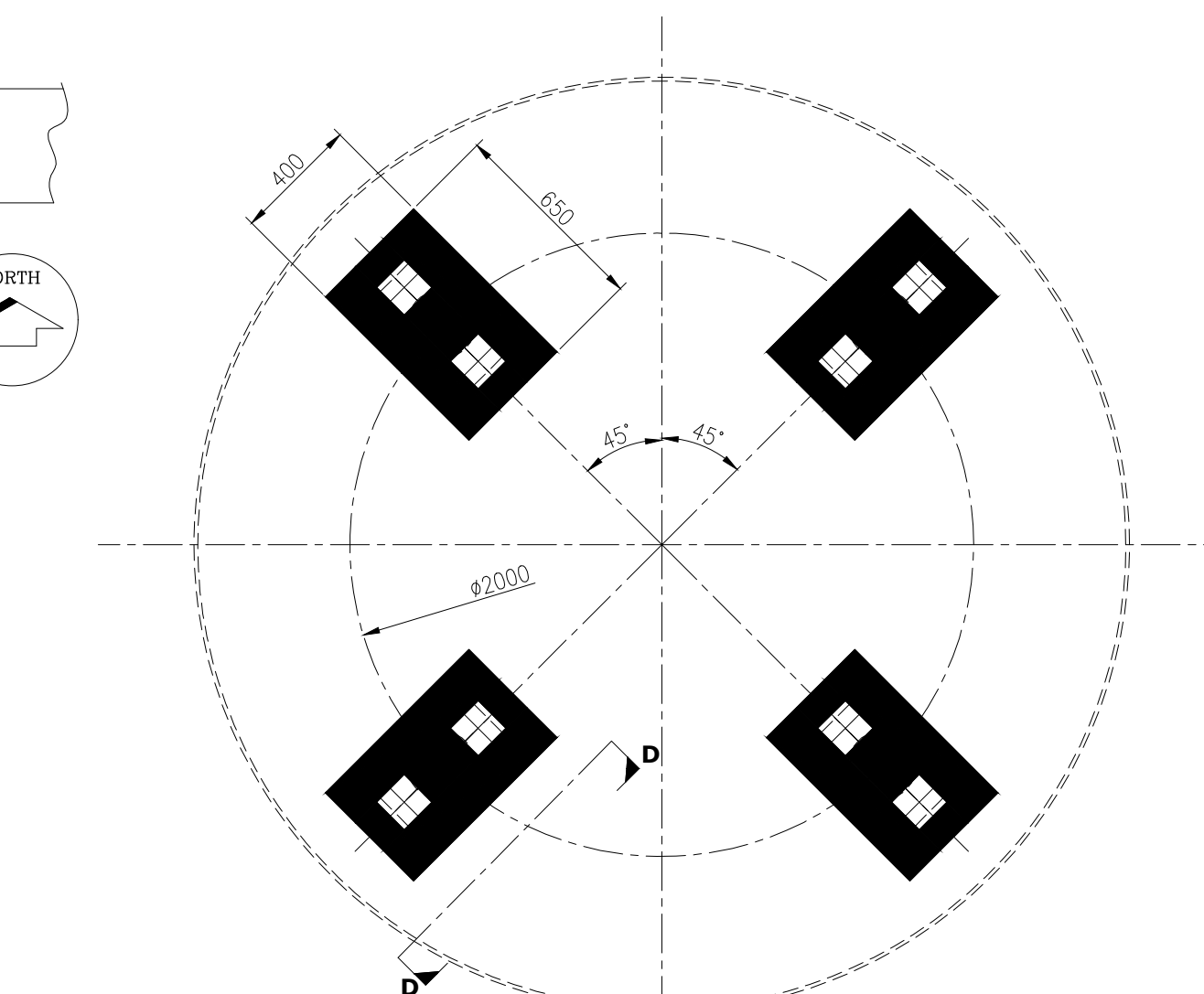
FOUNDATION PLAN
