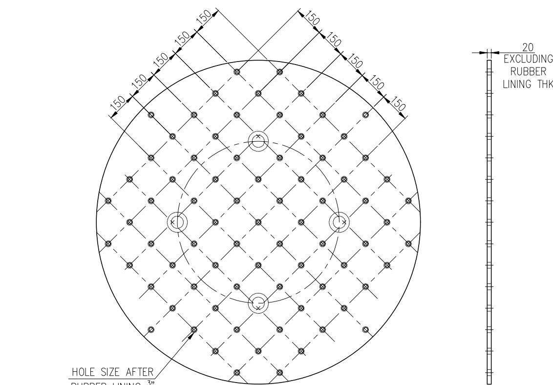
BOTTOM PLATE AND STRAINER DETAILS
