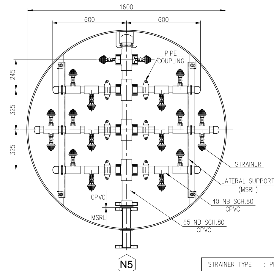
04 ALAKALI INLET HEADER AND STRAINER DETAILS
