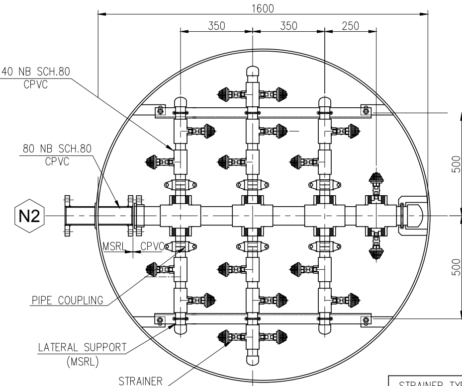
05 MIDDLE COLLECTOR AND STRAINER DETAILS
