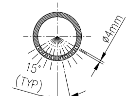
SECTION C-C
