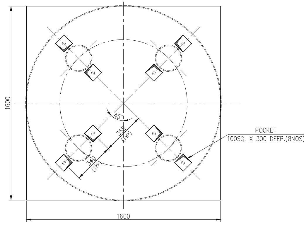
VESSEL FOUNDATION DETAILS
