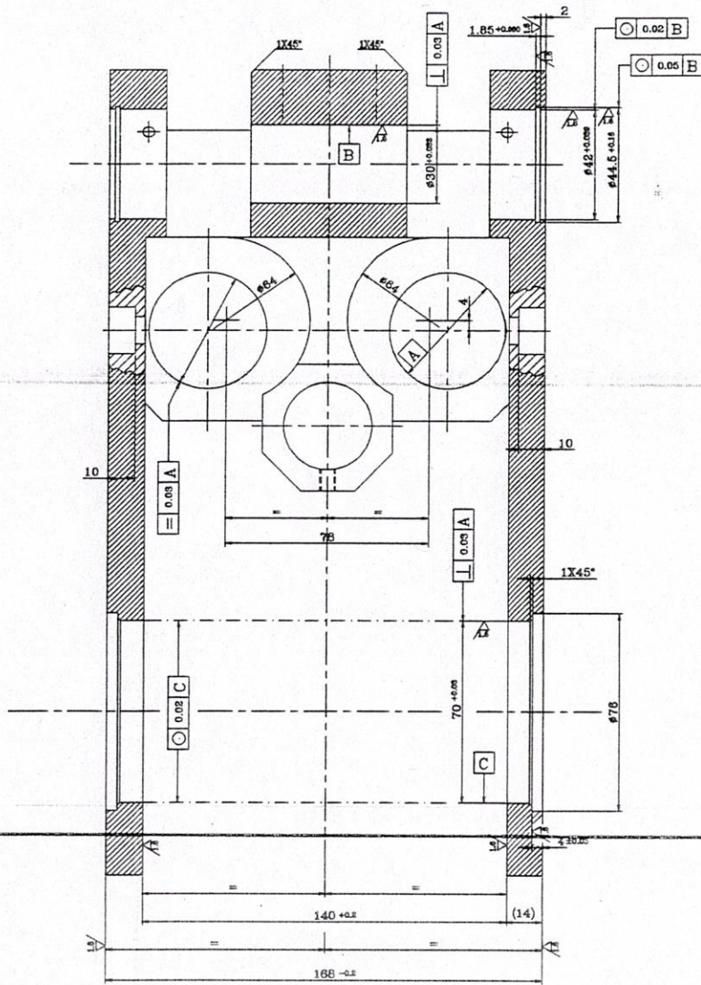
SECTION A-A ZONE M13, G13
