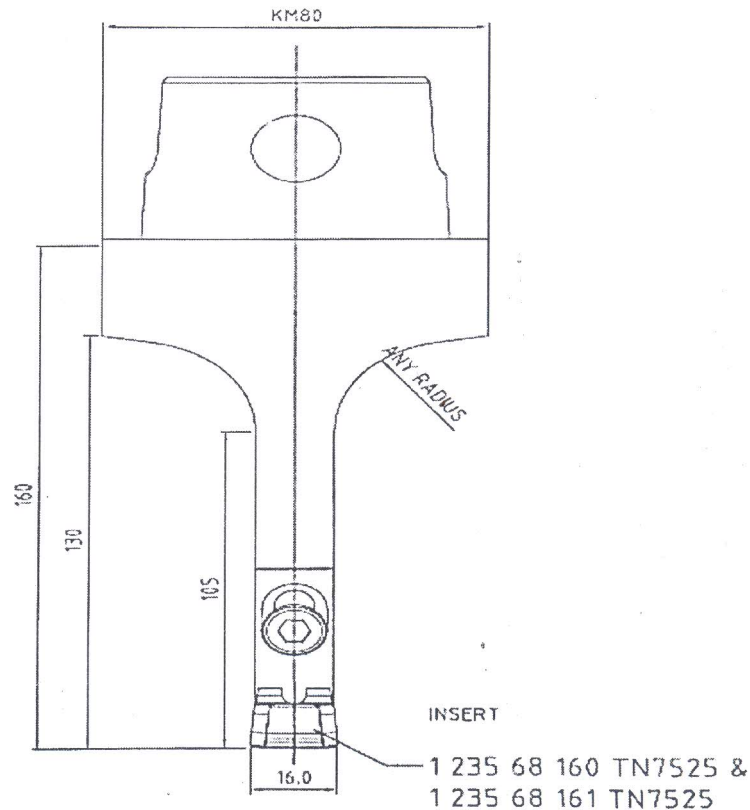
SCHEMATIC DRG 16MM TOOL
