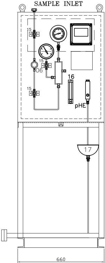
FRONT VIEW WITH OPENED GLASS DOOR
