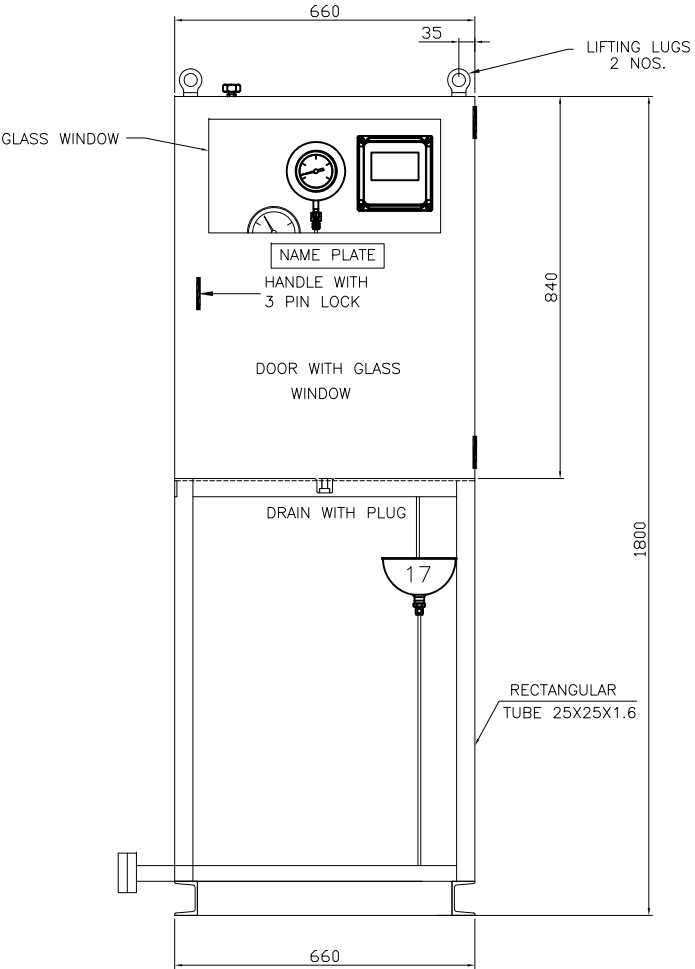
FRONT VIEW WITH CLOSED GLASS DOOR
