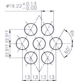
PITCH DETAIL (TOTAL No. OF HOLES - 4978)
