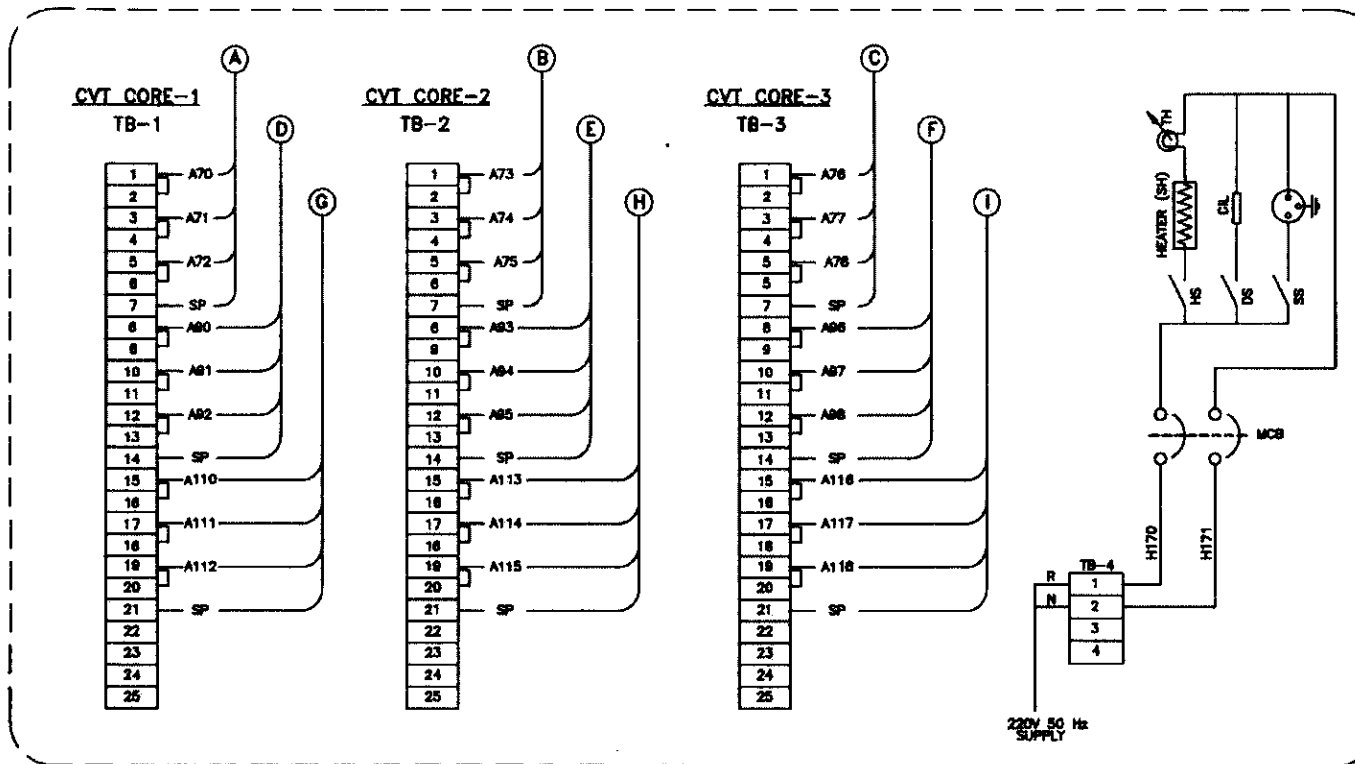
CVT MARSHALLING BOX
