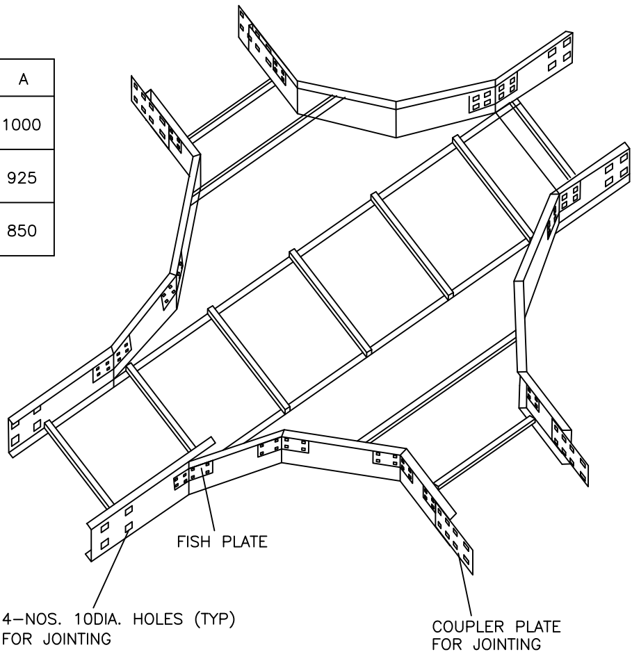
HORIZONTAL CROSS-PLAN
