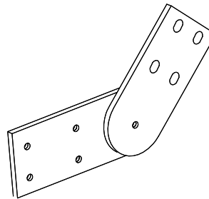
FRP ADJUSTABLE VERTICAL SPLICE PLATE
