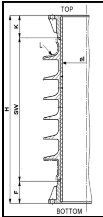
Figure 1: Typical Insulator Geometry for 245kV Composite Hollow Insulator
