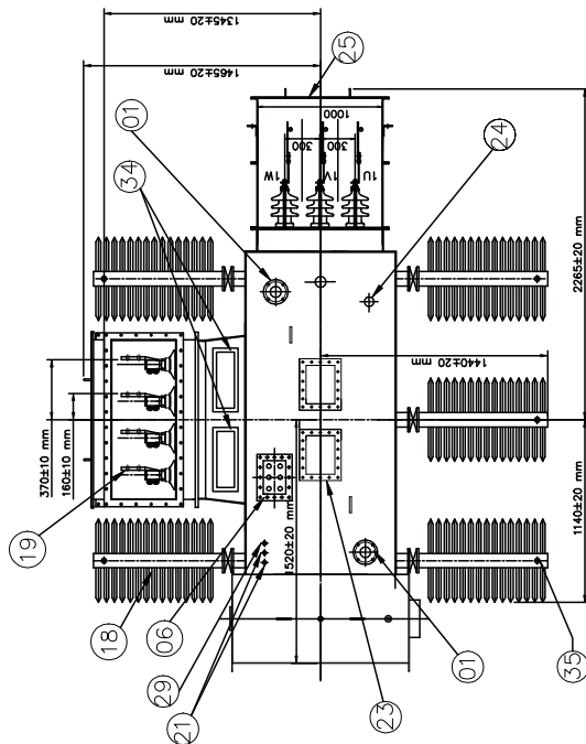
TOP VIEW DIRECTION OF WITHDRAWAL TRANSFORMER
