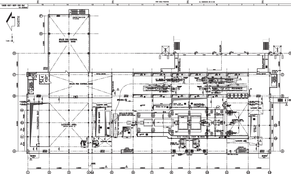
PLAN AT EL.17.0M
