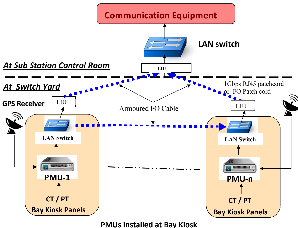
Fig 1.2: Typical Network Architecture at Sub Stations having Bay Kiosks at Switch Yard.
