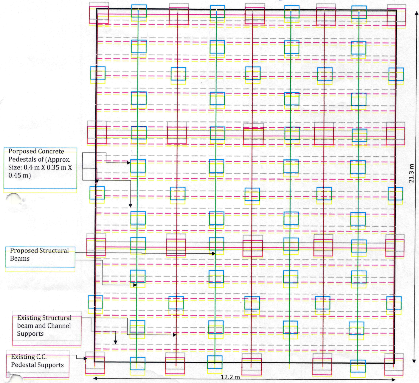
LAYOUT OF BASE FRAME FOR BHEL OFFICE (PORTA CABIN)
