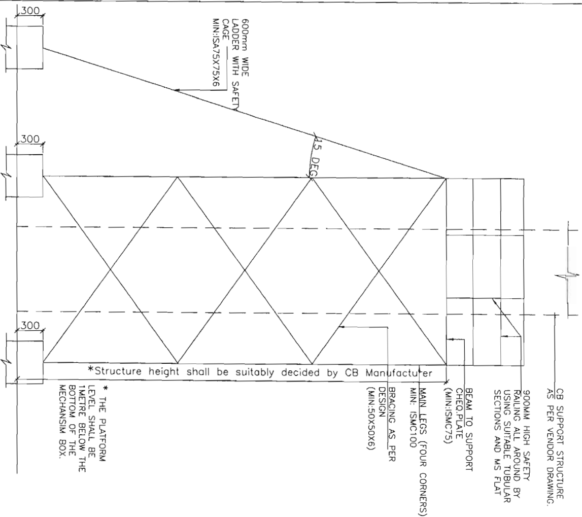
SECTION X-X
