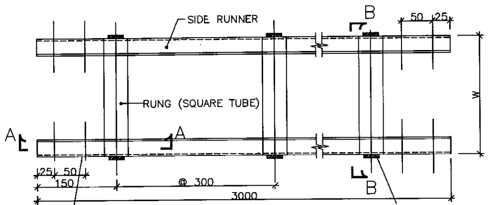
FRP LADDER TYPE CABLE TRAY
