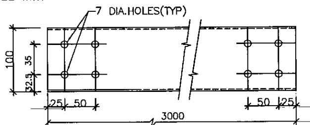
SIDE RUNNER
