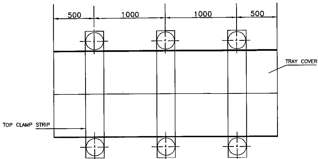
CABLE TRAY COVER WITH ACCESSORIES -PLAN
