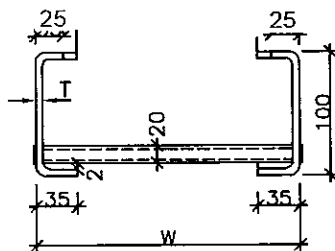
SEC-BB
