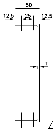
SECTION-CC (100/50 TRAYS)
