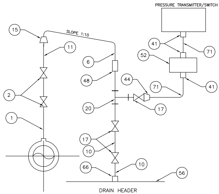
TRANSMITTER MOUNTED ABOVE INSTRUMENT SOURCE POINT FIG-C
