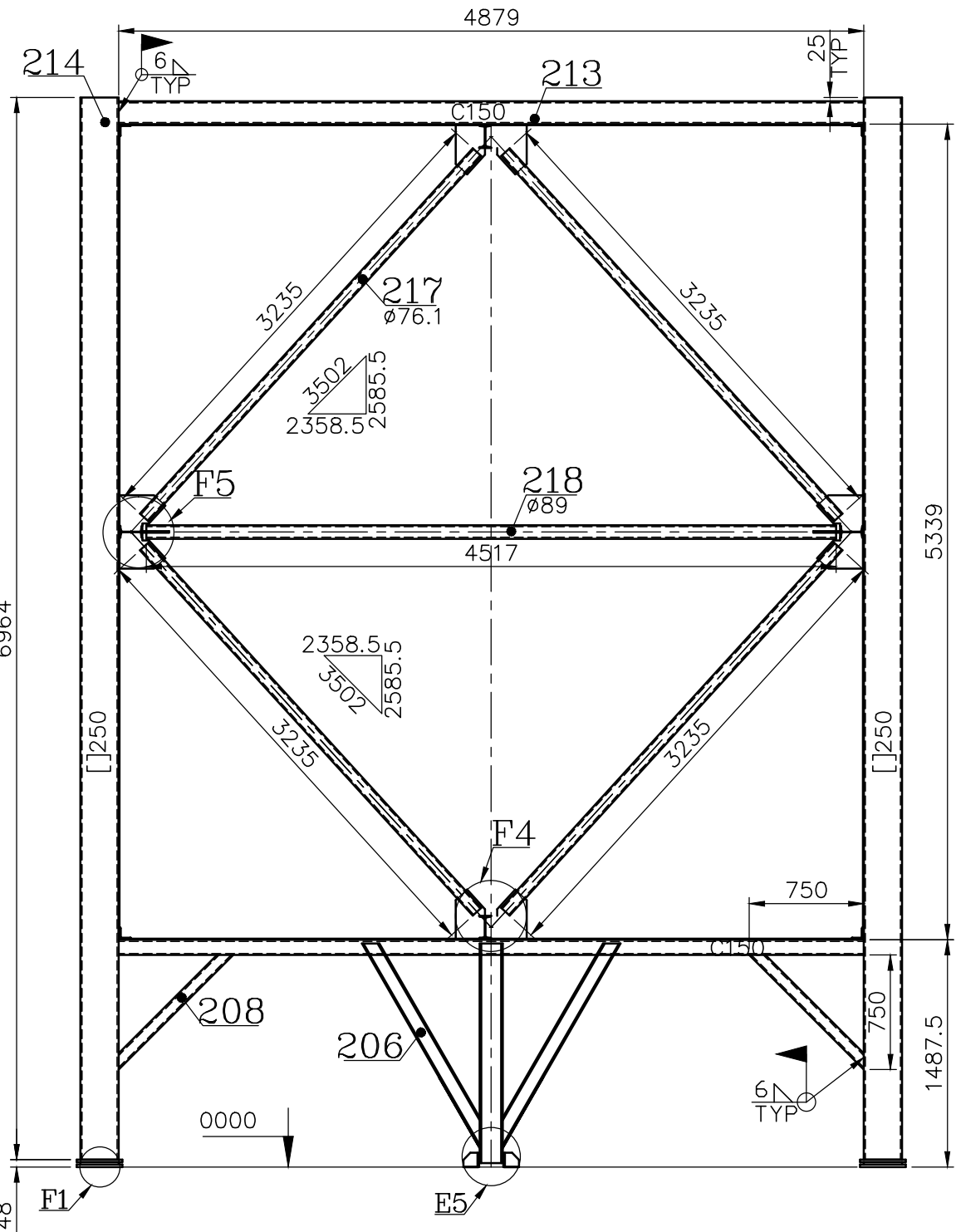
SECTION-FF (2 PLACES) (REF SH 01)
