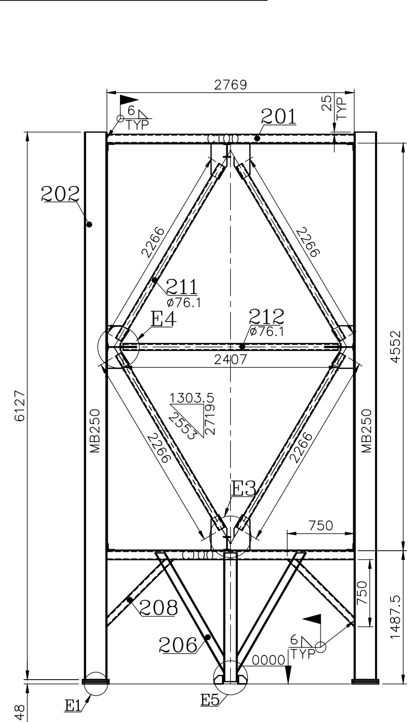
SECTION-EE (2 PLACES) (REF SH 01)
