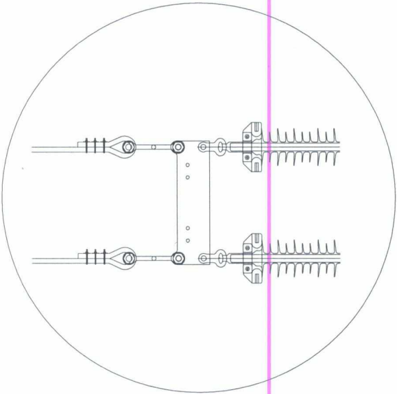
ANCHORING DETAILS
