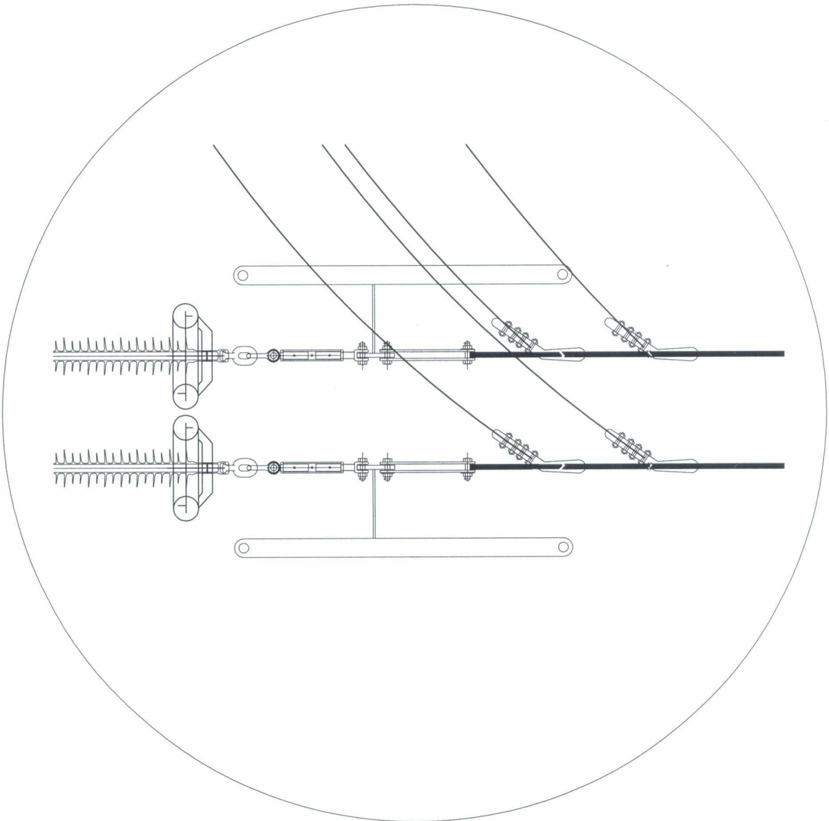
CONNECTION ARRANGEMENT
