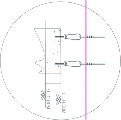
FOUNDATION DETAILS
