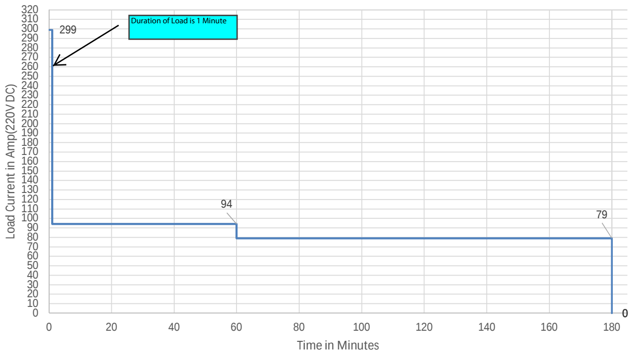
Battery Load Cycle - 220V
