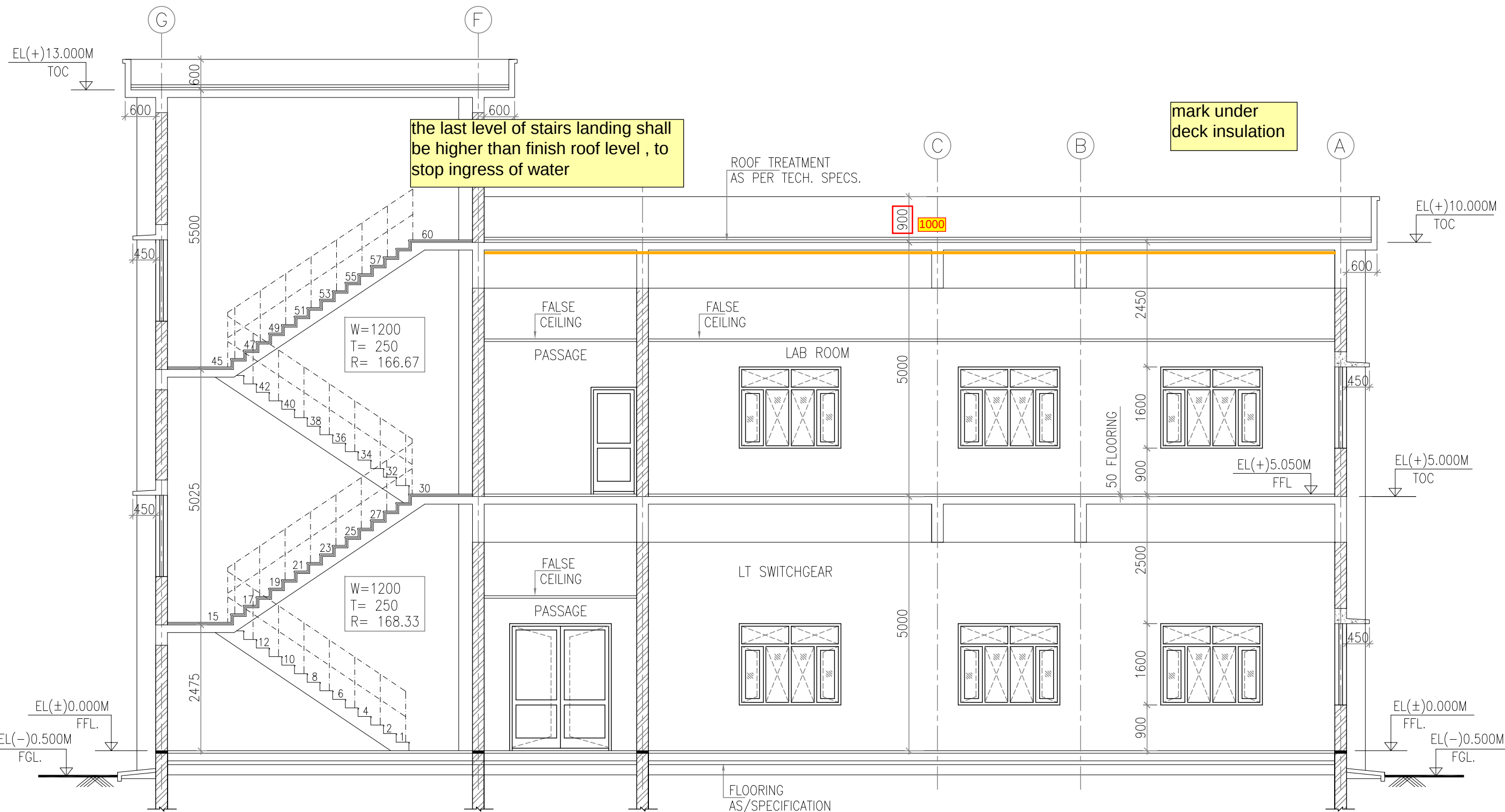
SECTION B-B
