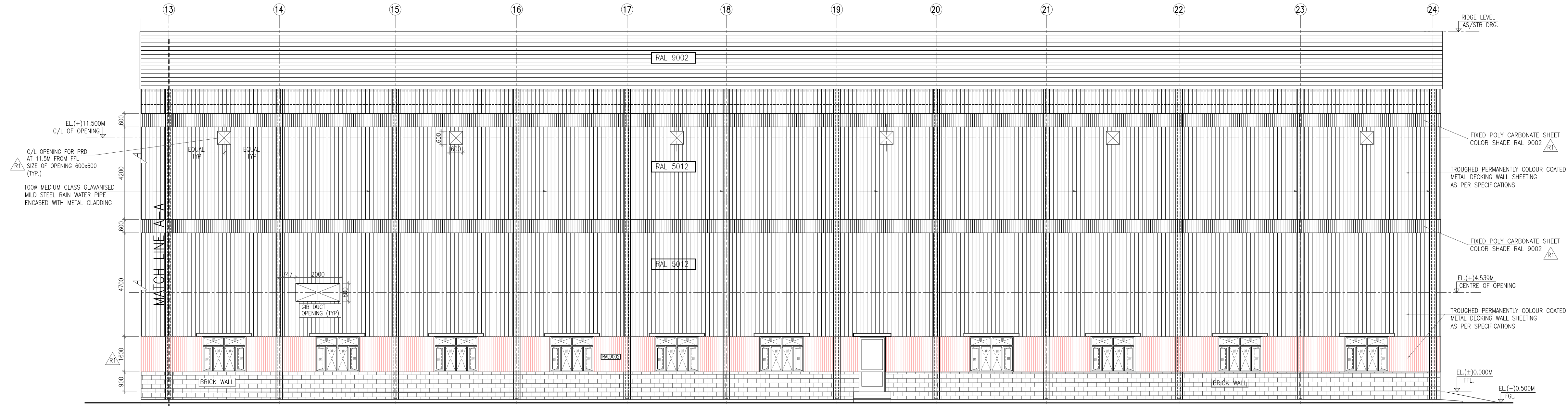
ELEVATION ALONG GRID-D
