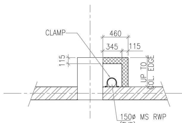
TYP. RWP FIXING DETAIL
