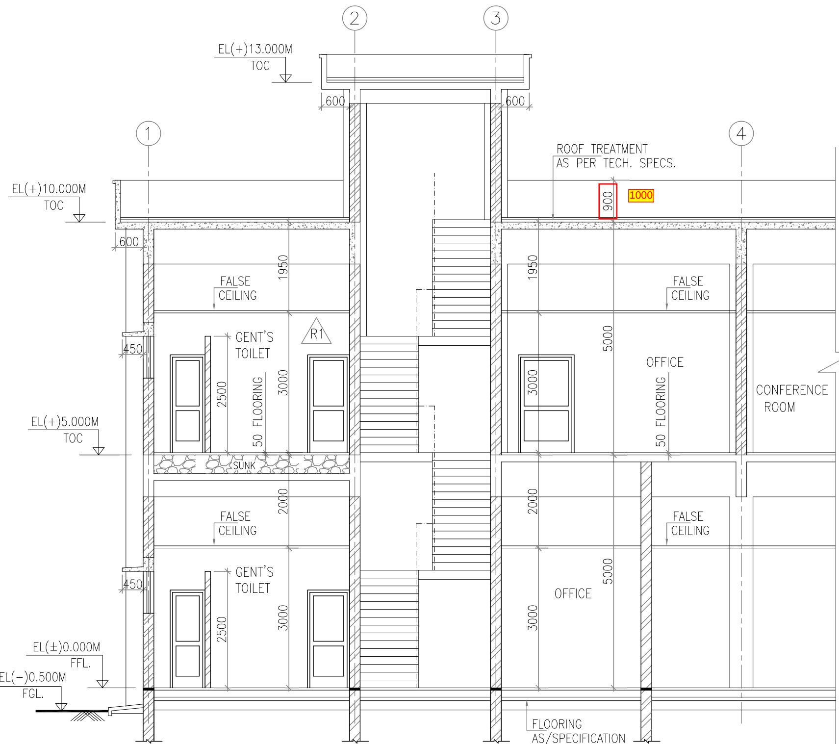
SECTION C-C
