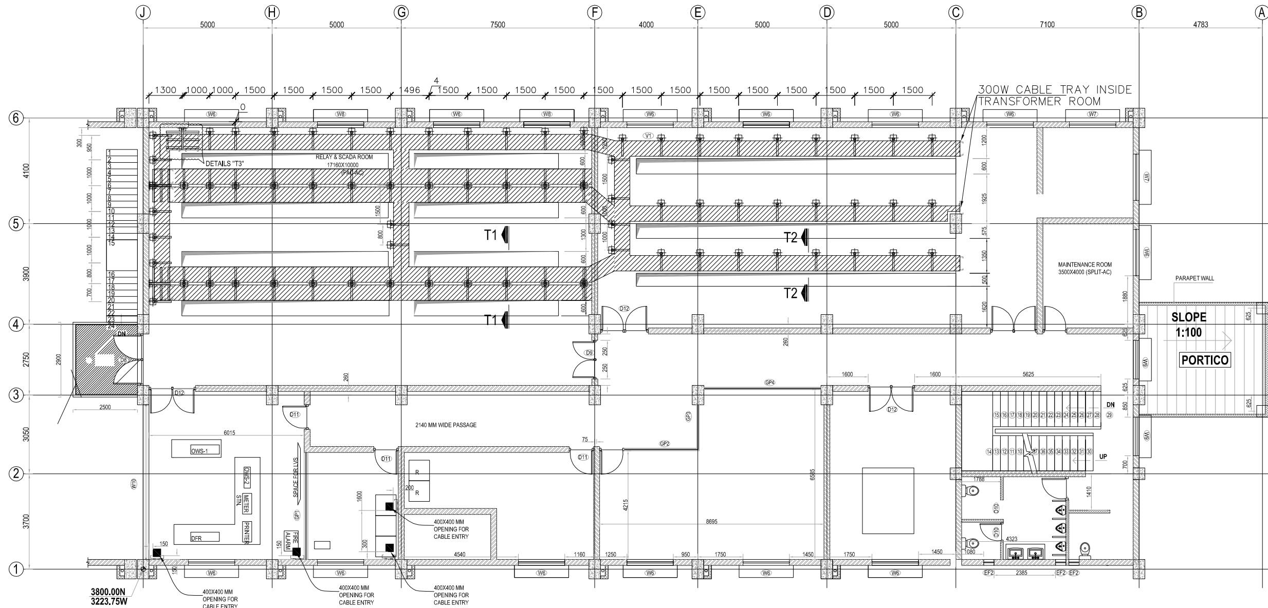
CABLE HANGER / TRAY MOUNTING ARRANGEMENT UNDER GROUND FLOOR ROOF SLAB
