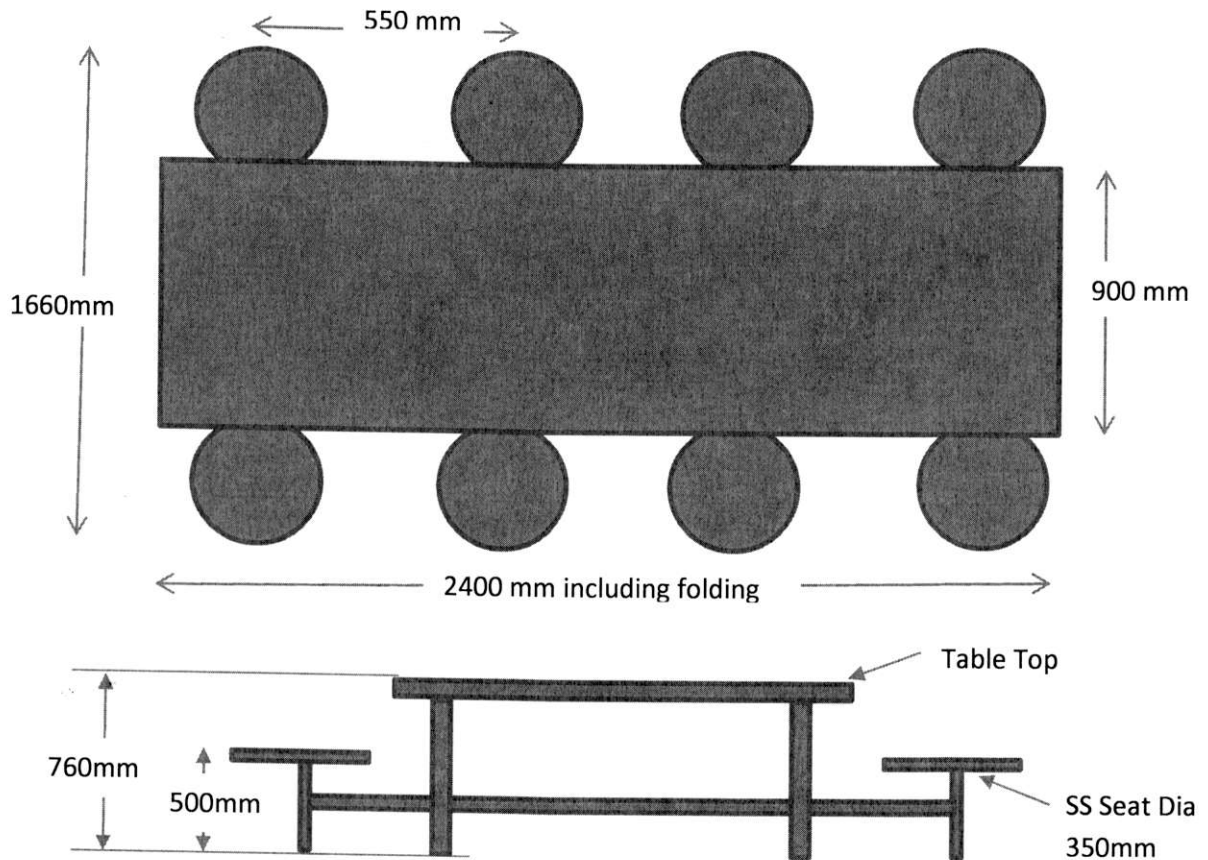
Fig.2 Typical Dimensions Dining table (8 seats)
