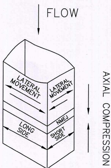
VERTICAL DUCT
