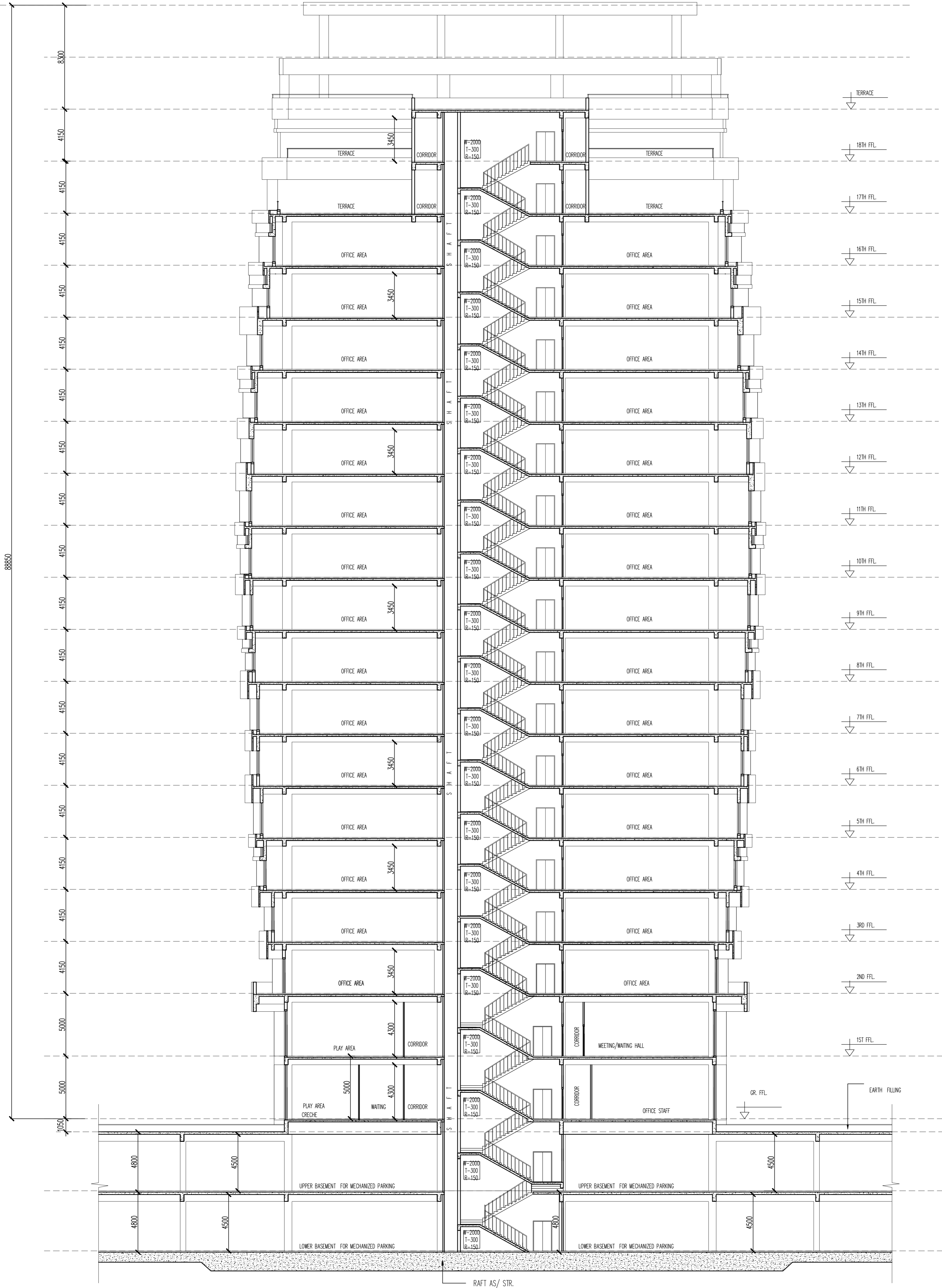
SECTION 2-2
