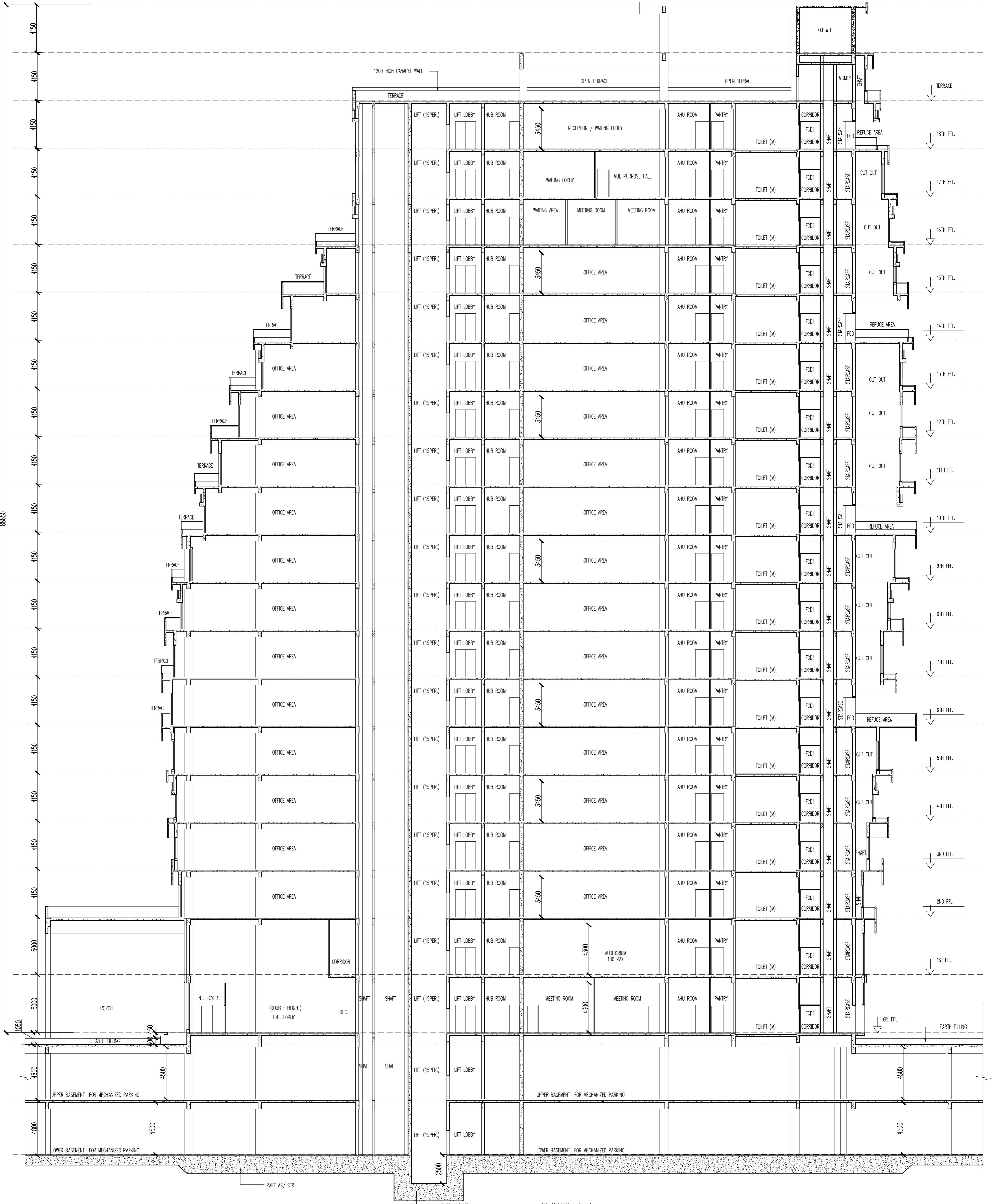
SECTION 1-1
