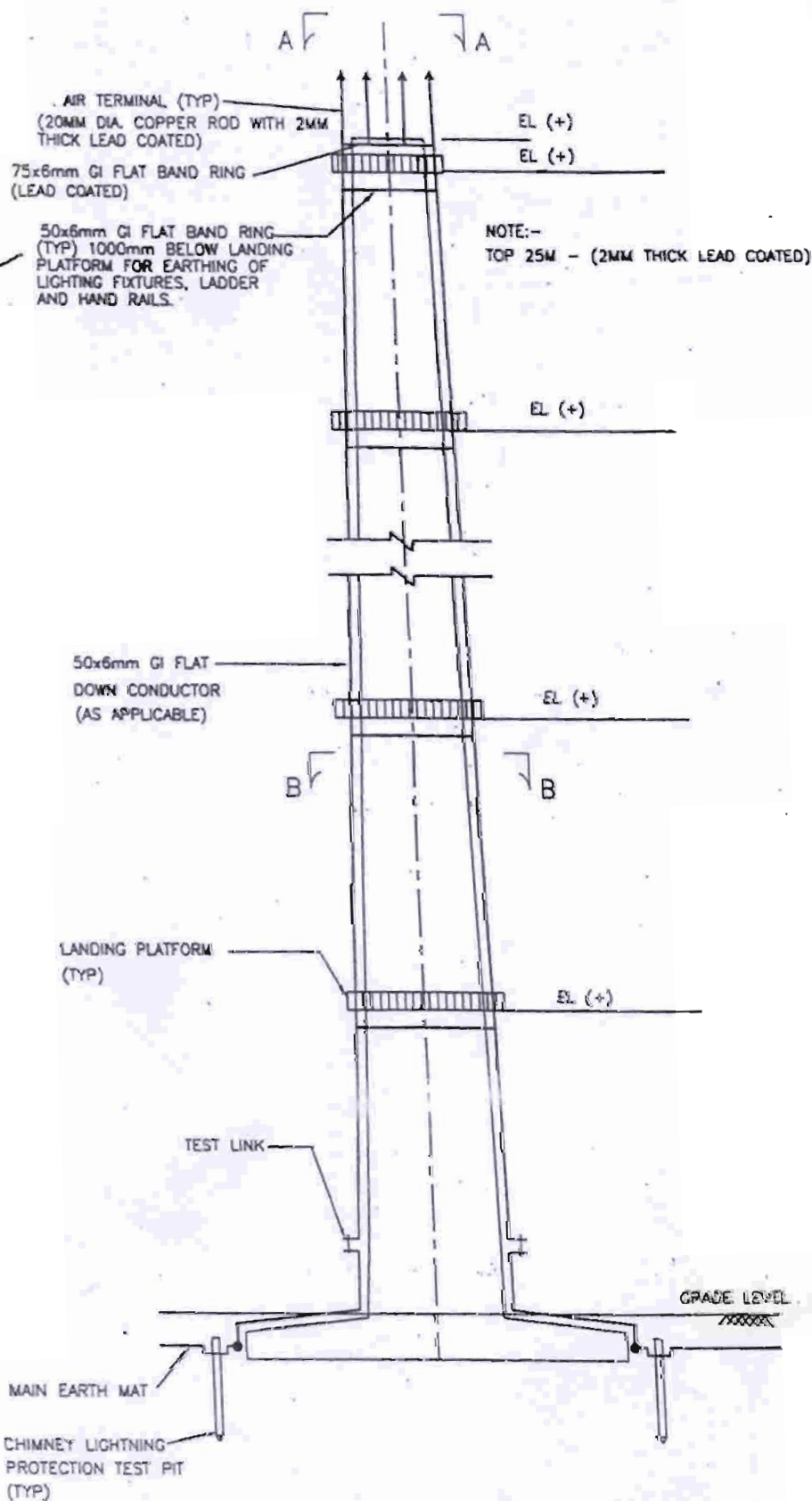
CHIMNEY (ELEVATION)
