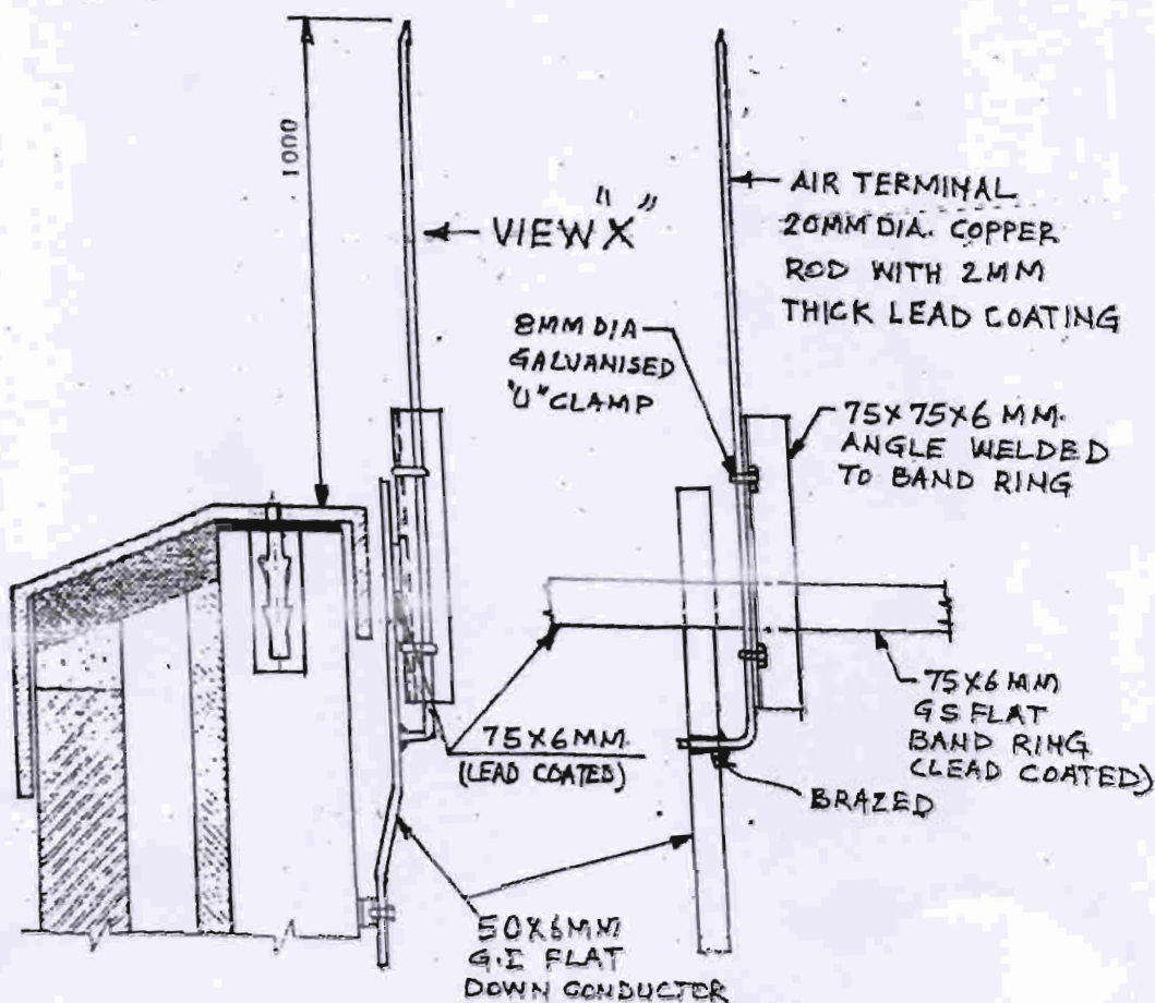
SECTION 2-2
