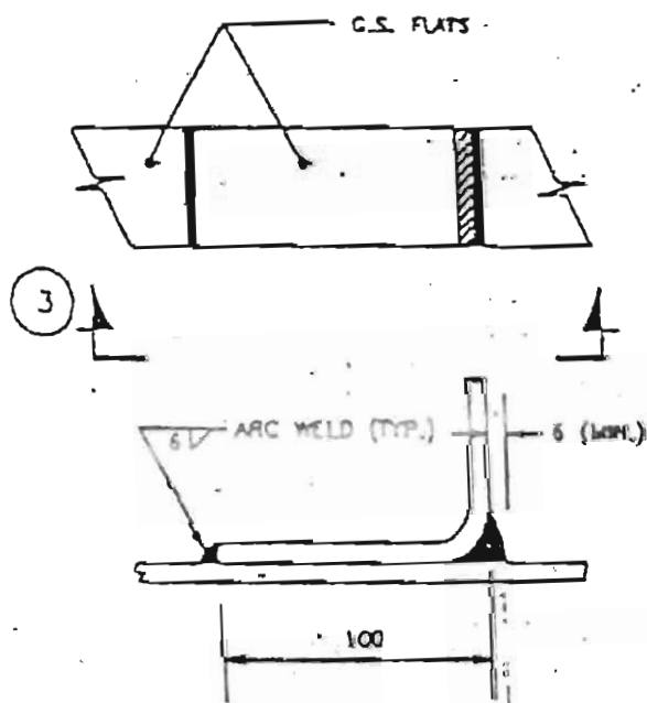
ANGULAR JOINT BETWEEN G. S. FLATS
