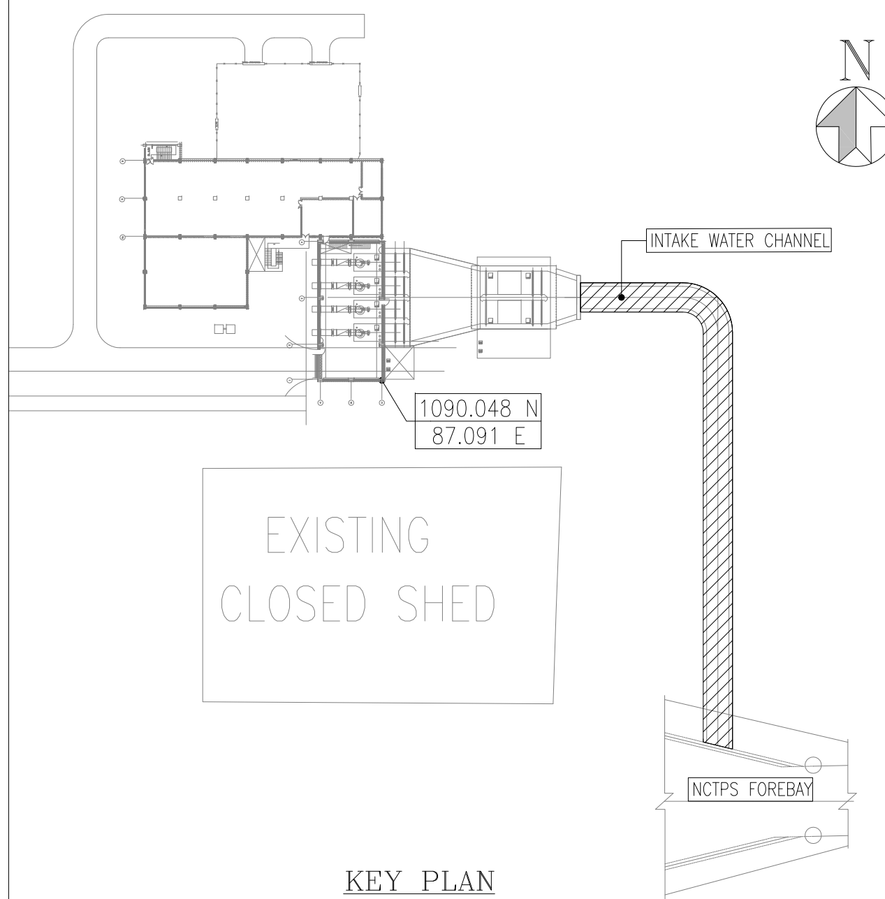
KEY PLAN
