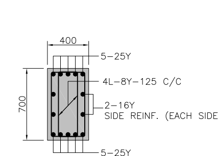
SECTION 2-2
