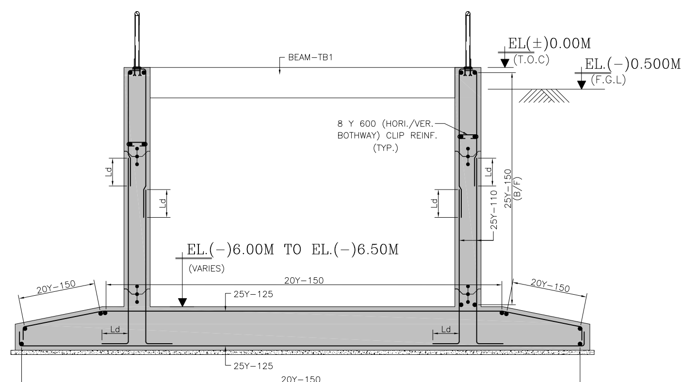
SECTION 1-1 (REINF. DETAIL)
