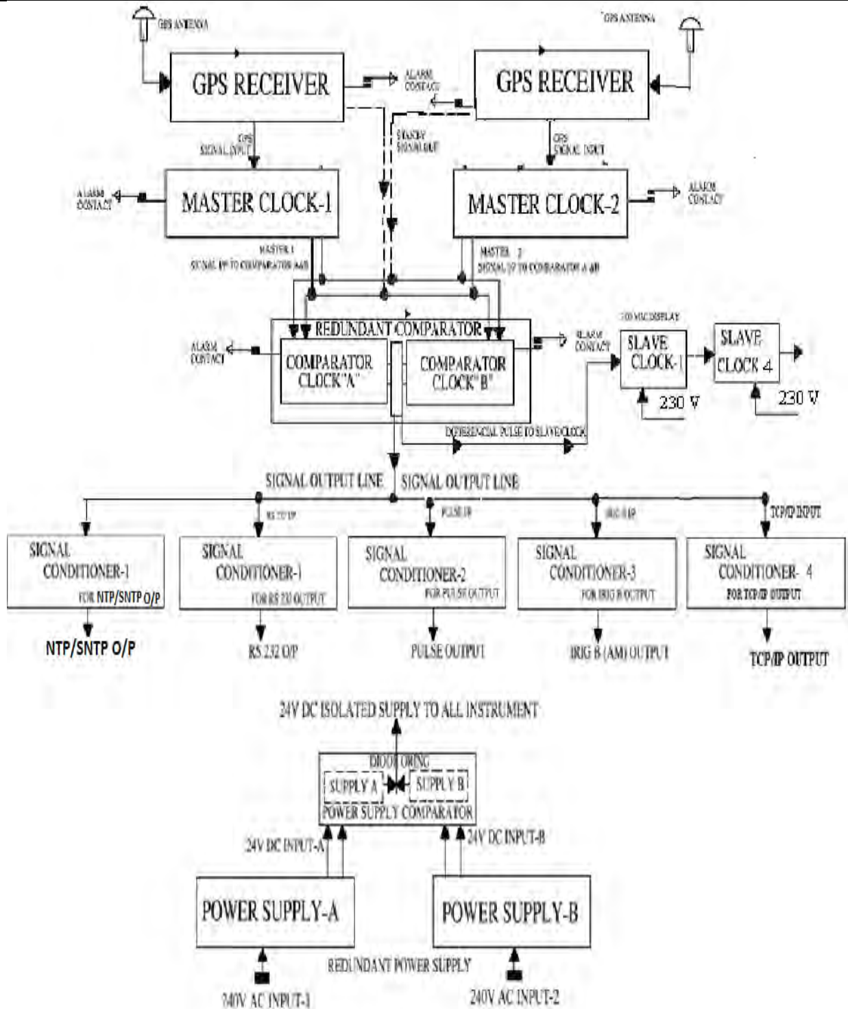
Fig 1: TYPICAL CONFIGURATION DIAGRAM
