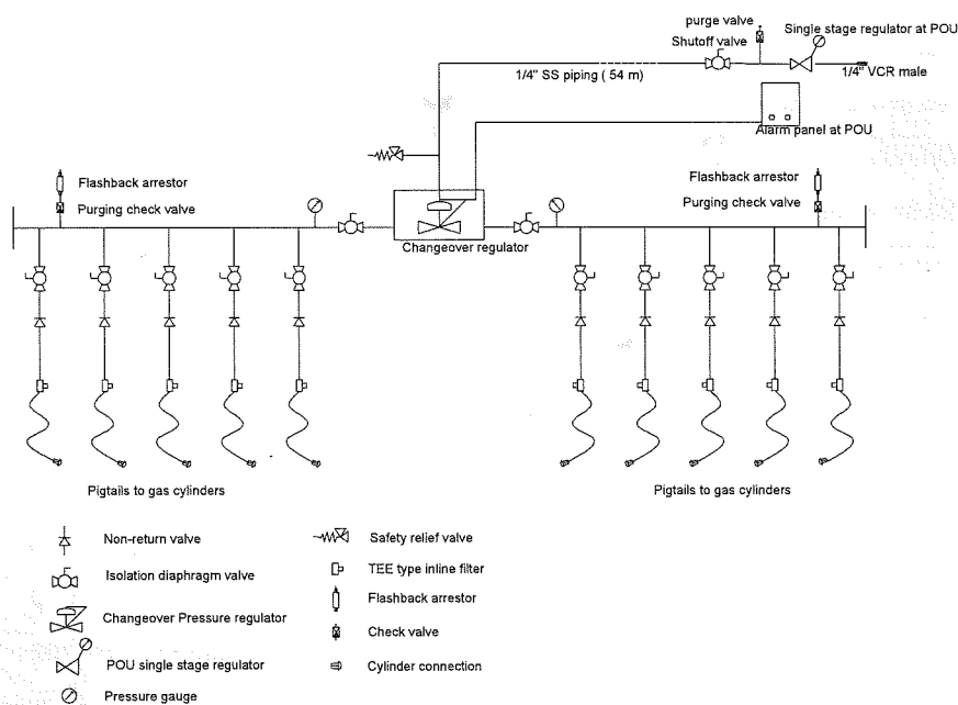
(a) Schematic of the manifold and piping
