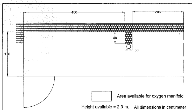
(b) Layout of the area available for manifold
