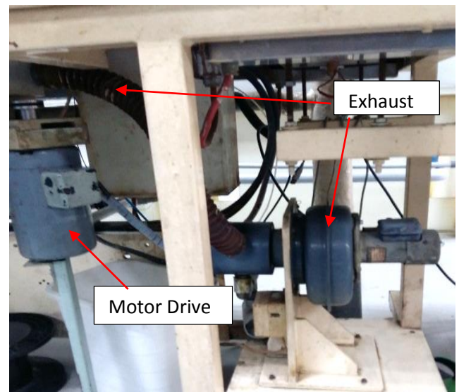
PICTURE-5: EXHAUST
