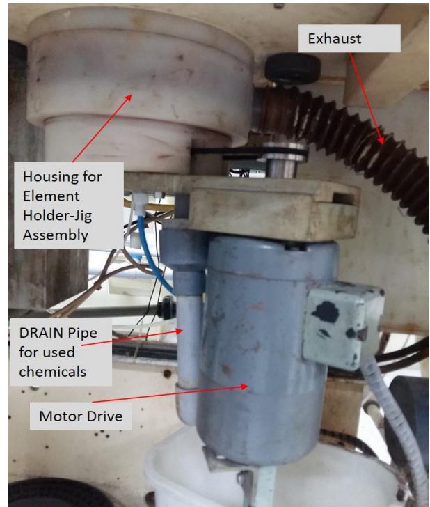
PICTURE-4: MOTOR DRIVE ASSEMBLY
