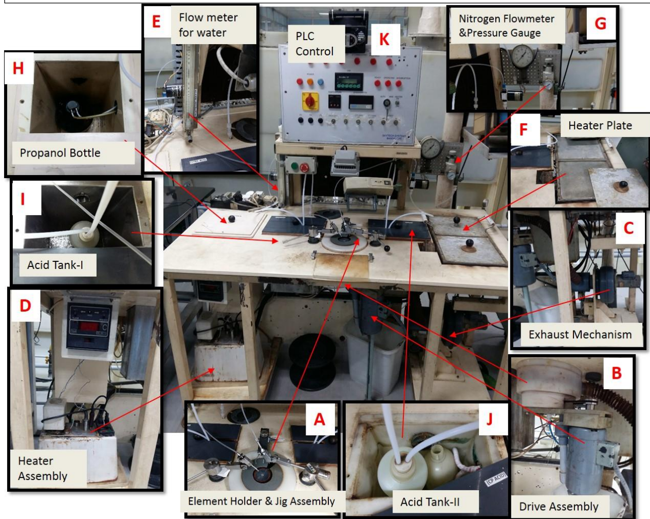
PICTURE-1: BEVEL ETCHING MACHINE
