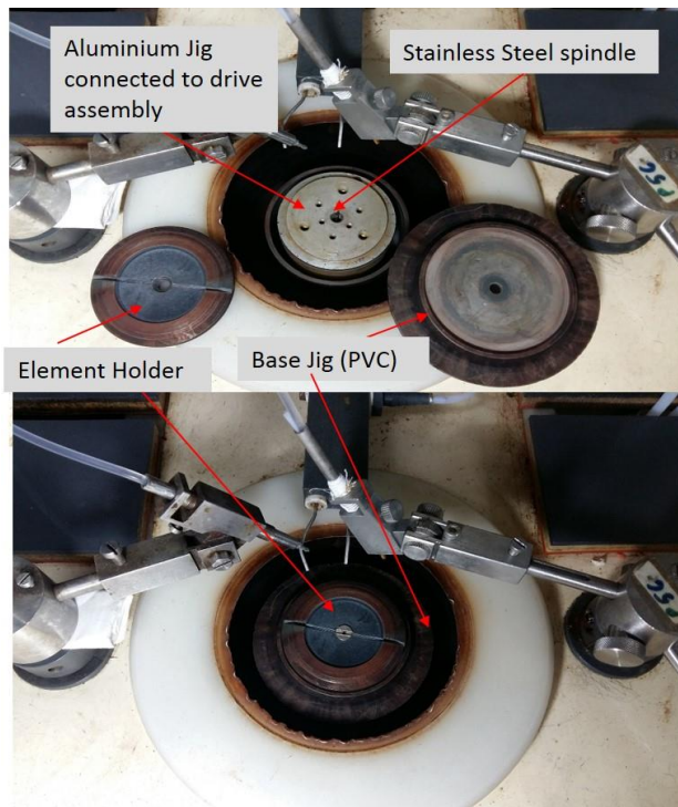
PICTURE-3: ELEMENT HOLDING JIGS ASSEMBLY
