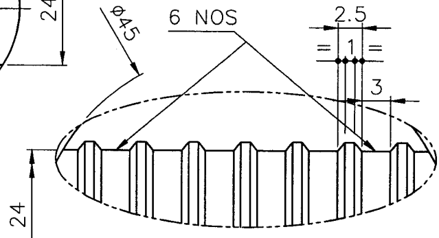
SLOT DETAIL
