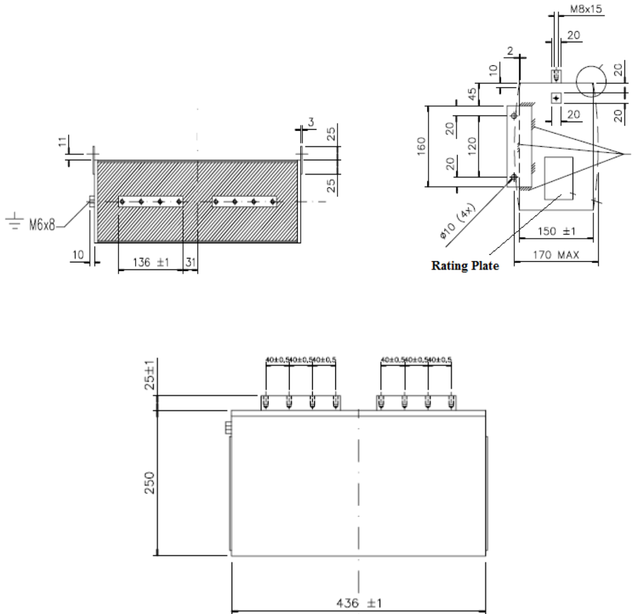
Fig 2: Dimensional Drawing
