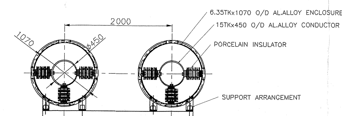
CROSS SECTION OF DELTA RUN BUSDUCT
