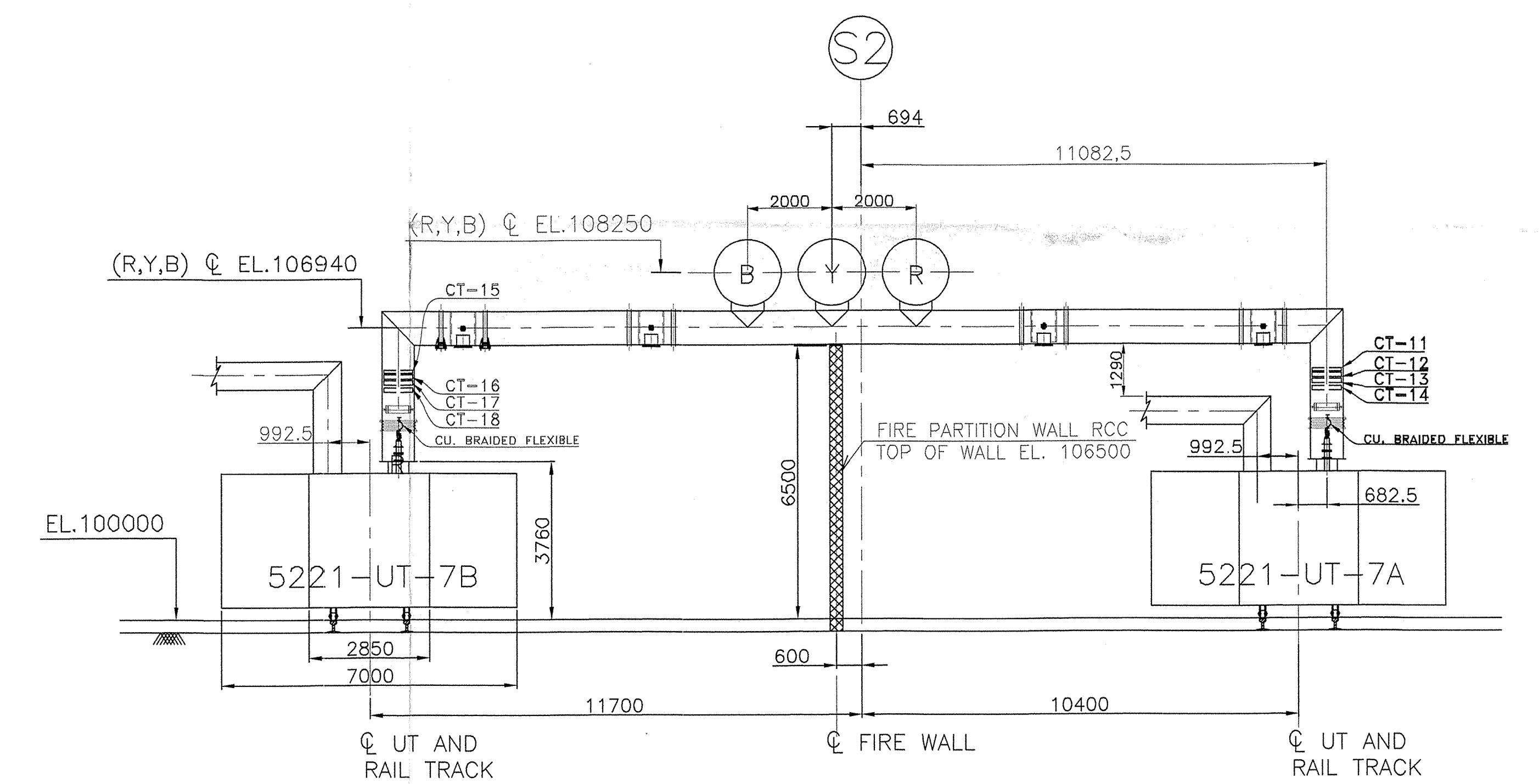
SECTION '4-4'
