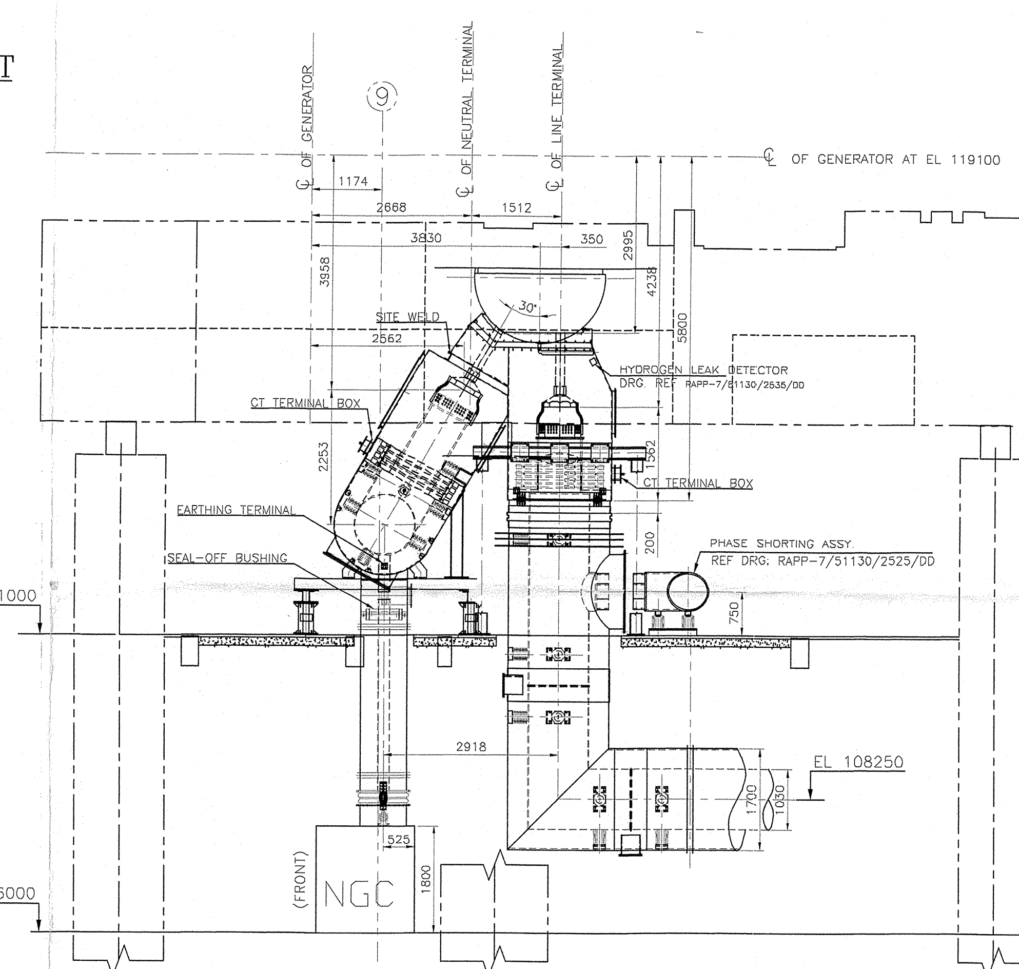
SECTION '2-2'
