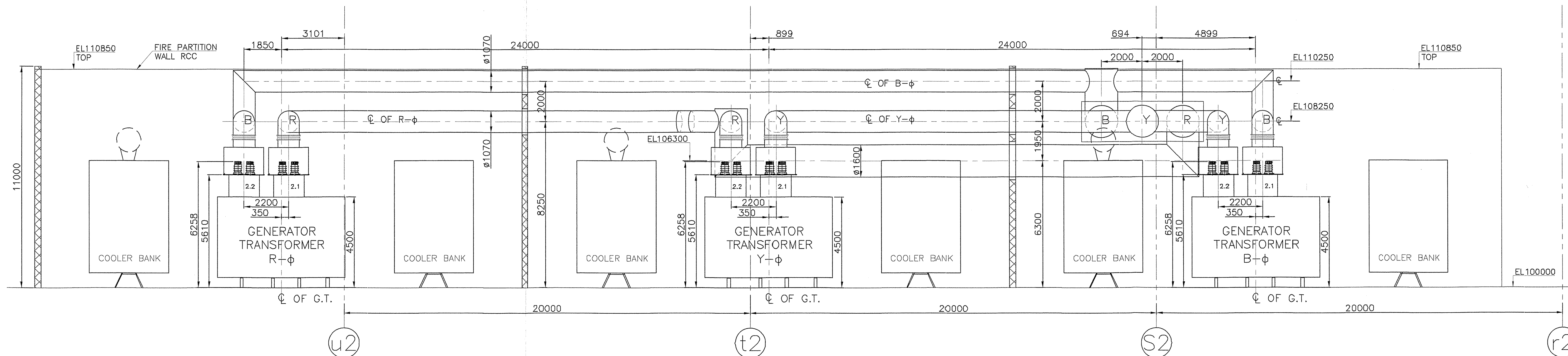
SECTION '3-3'
