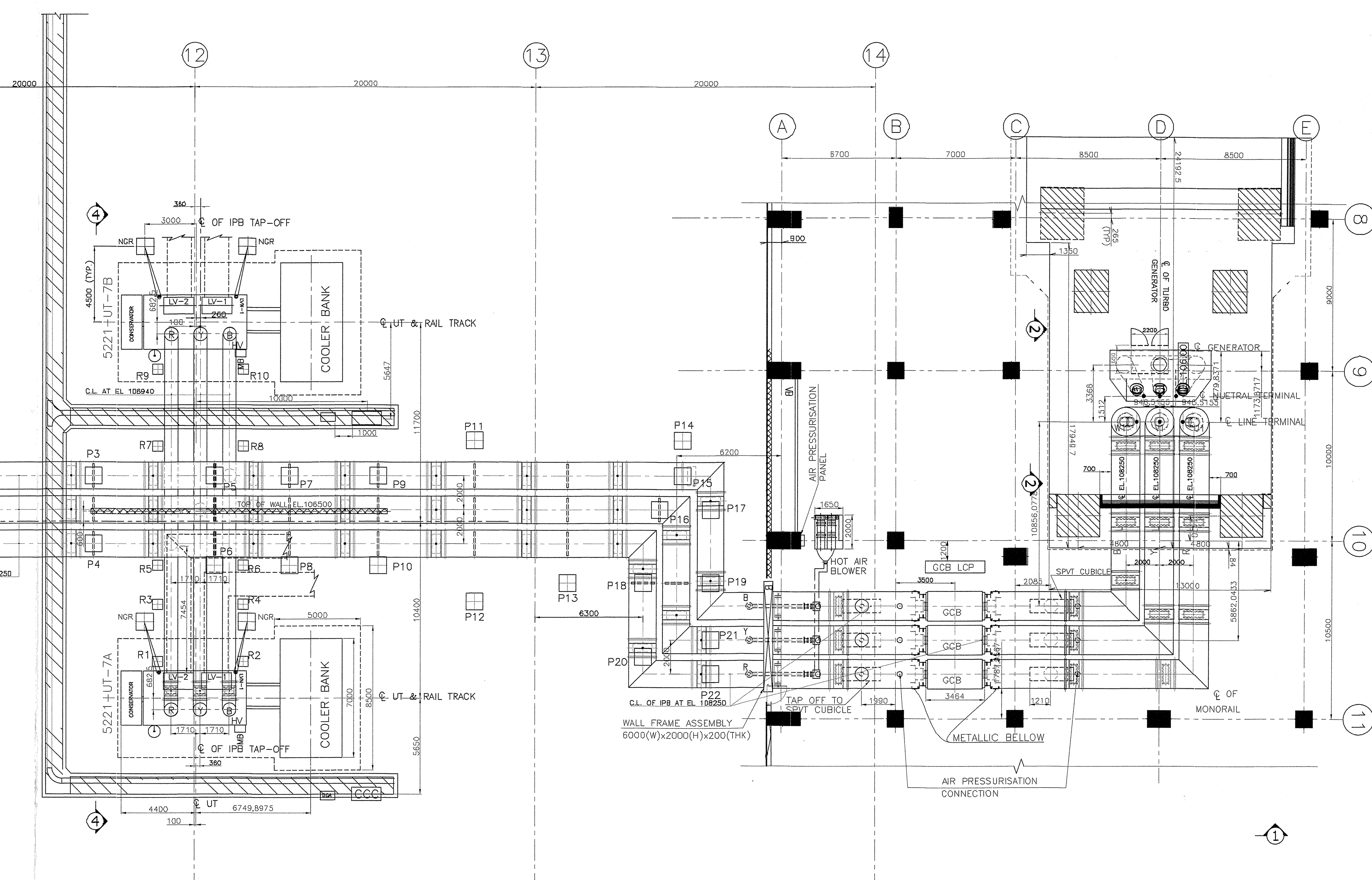
PLAN VIEW
