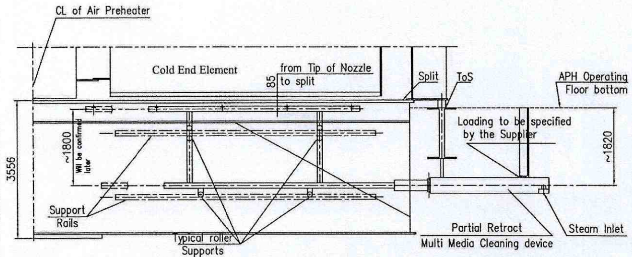
Partial Elevation
