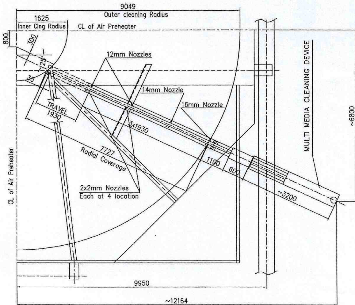
Plan View
