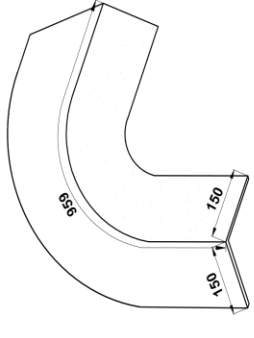
NORTHLIGHT CURVE LEFT BARGE BOARD (PROFILE TO MATCH NORTH LIGHT CURVE)
