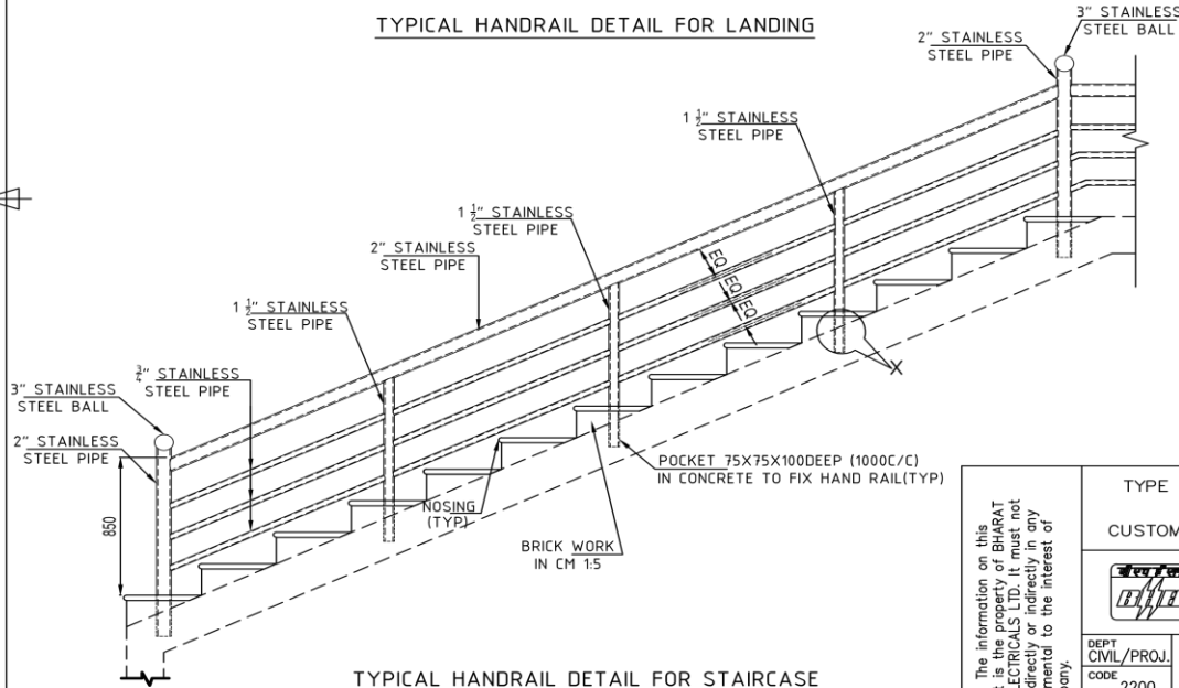
TYPICAL HANDRAIL DETAIL FOR STAIRCASE
