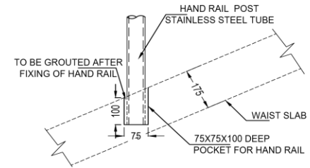
DETAIL-X DETAILS OF POCKETS FOR HAND RAIL
