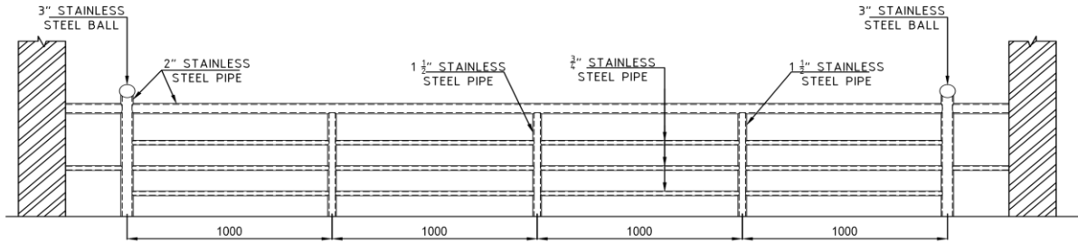
TYPICAL HANDRAIL DETAIL FOR LANDING
