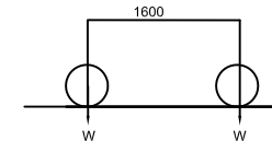
LT WHEEL LOAD WITH OUT IMPACT (W=4.2 T)
