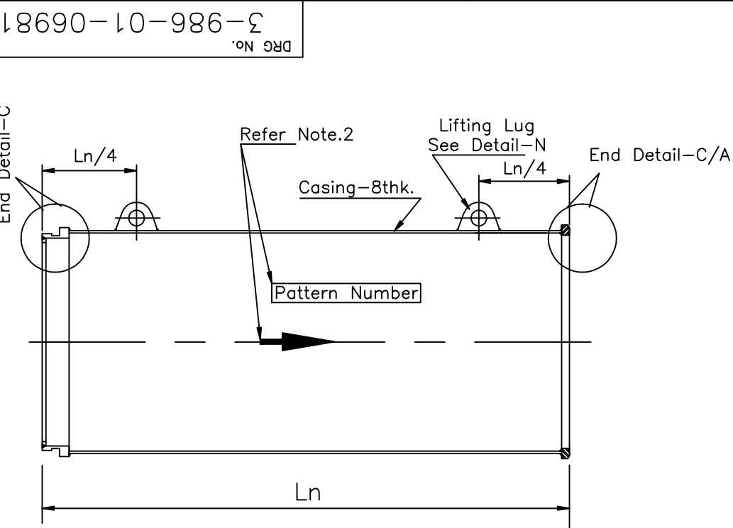
Section Of the M.S. Pipe (General Arrangement)
