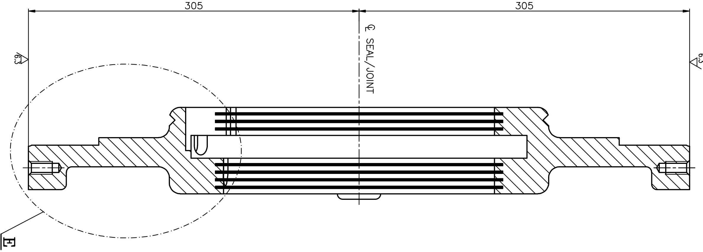
SECTION C-C
