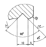
DETAIL - G (G12) 2:1
