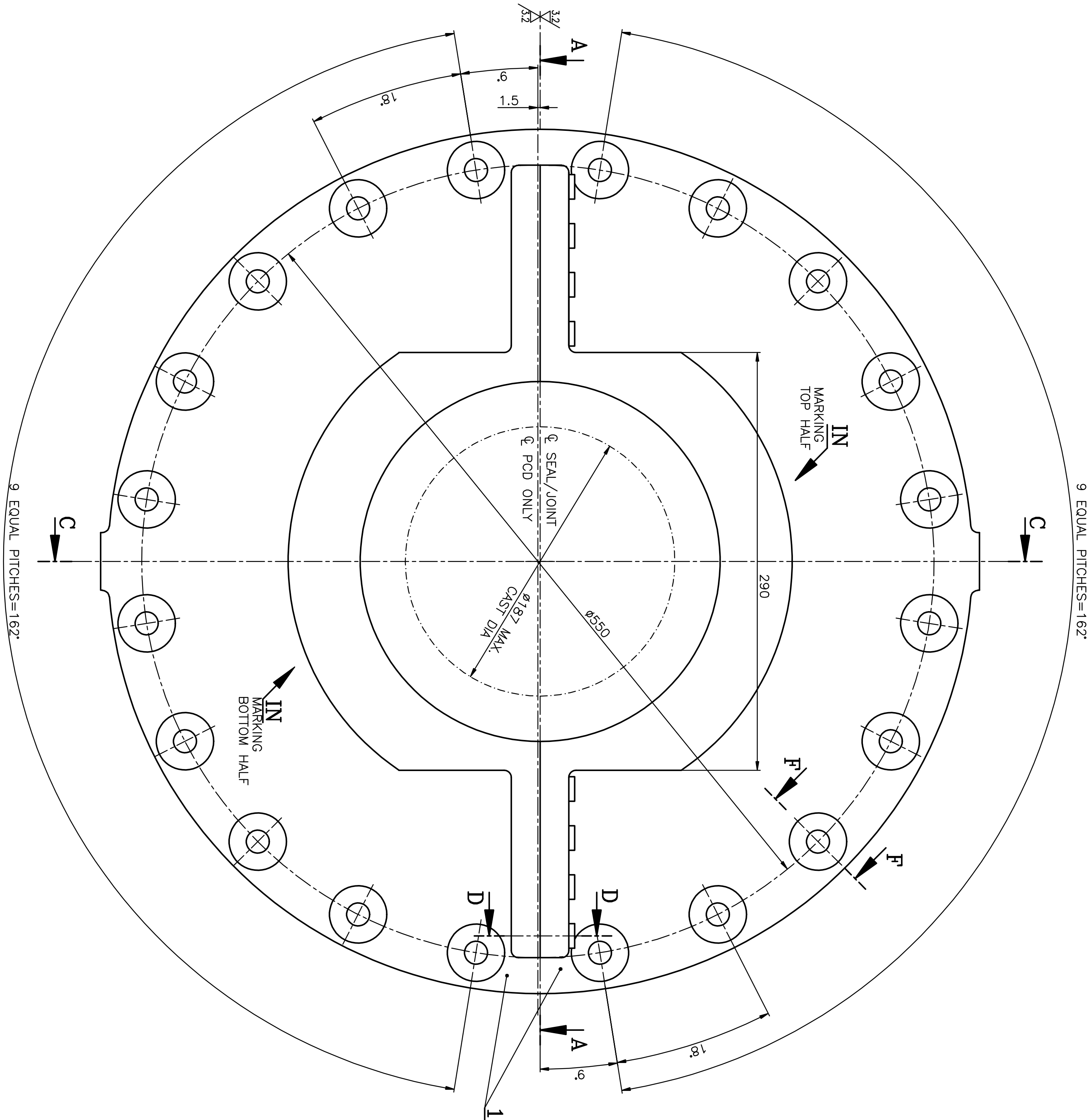
SEALING RING IN TWO PARTS
